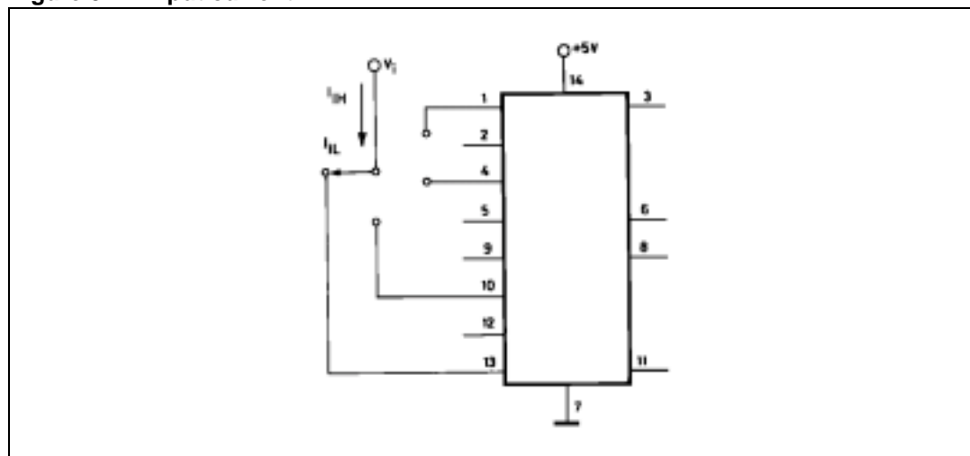
Figure 5. Input current
