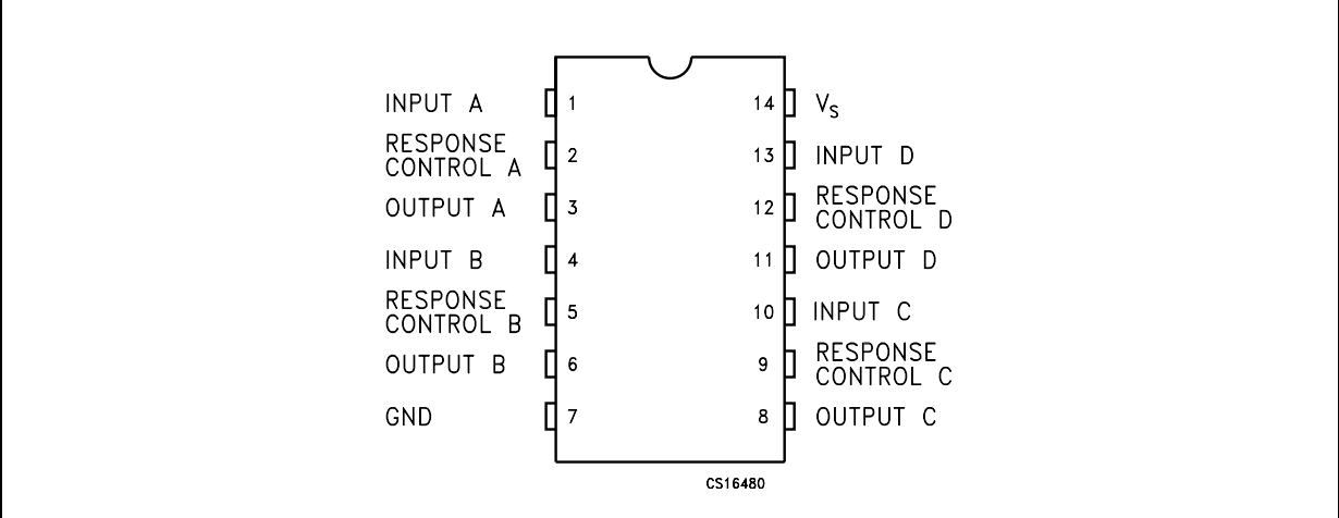
Figure 2. Pin connections
