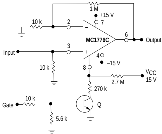
Figure 16. Gated Amplifier
