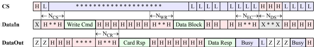
Figure 7-22 : SPI Single Block Write
