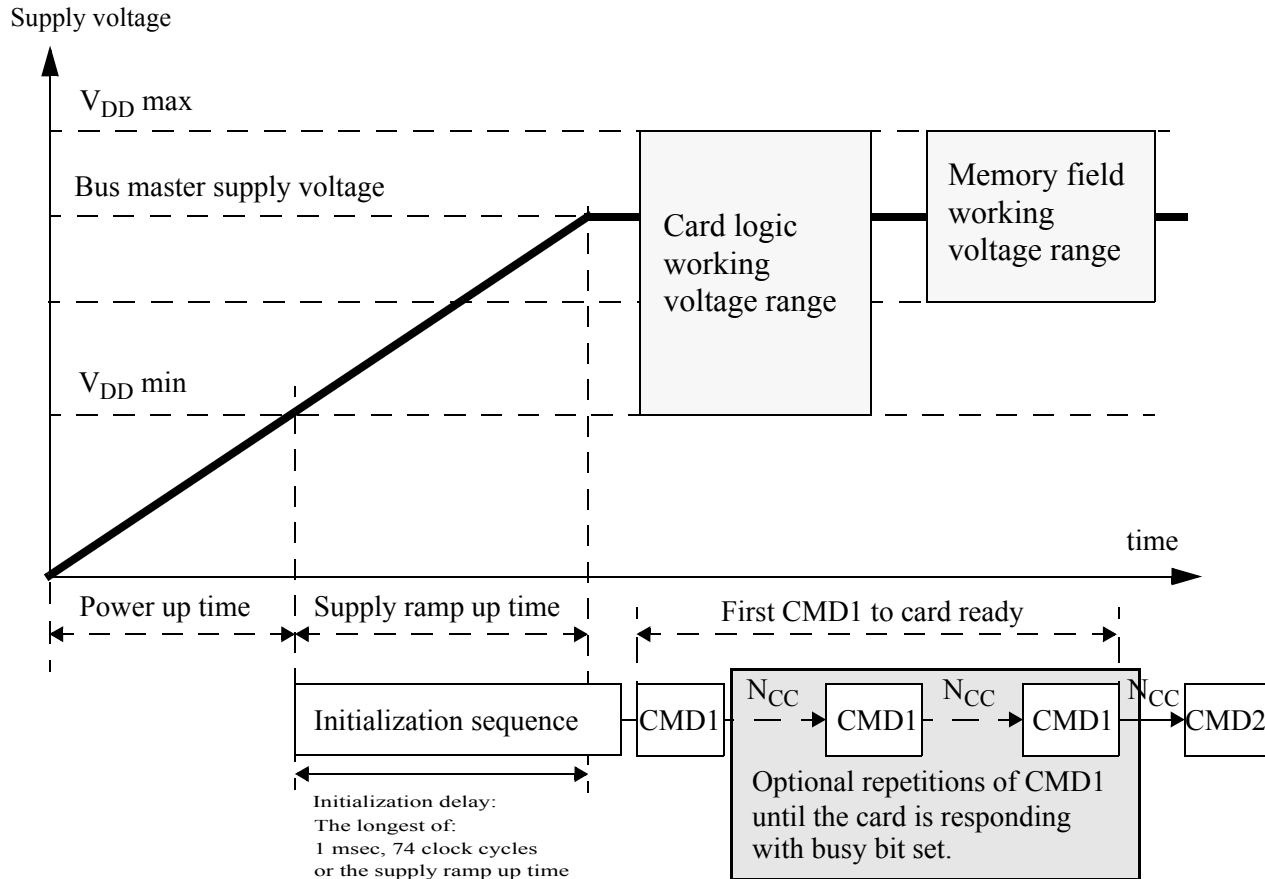
Figure 5-3 : Power-up Diagram
