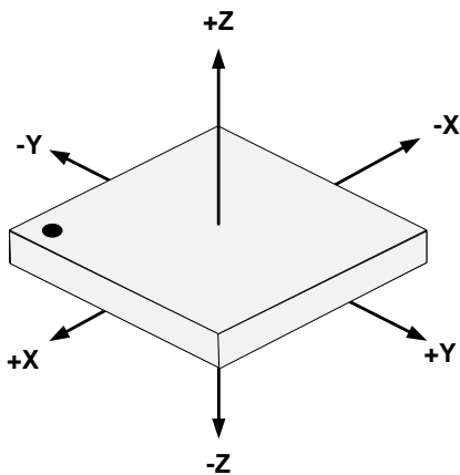
Figure 19. Package Axis Reference
