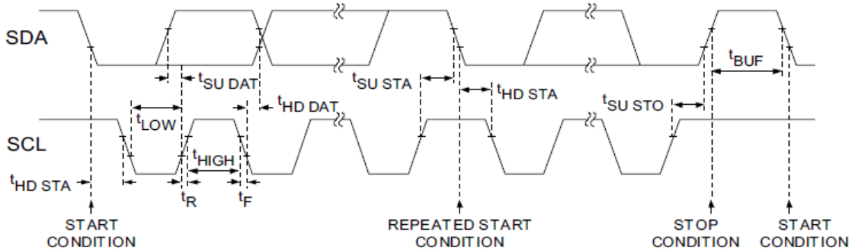
Figure 4. I2C Interface Timing
