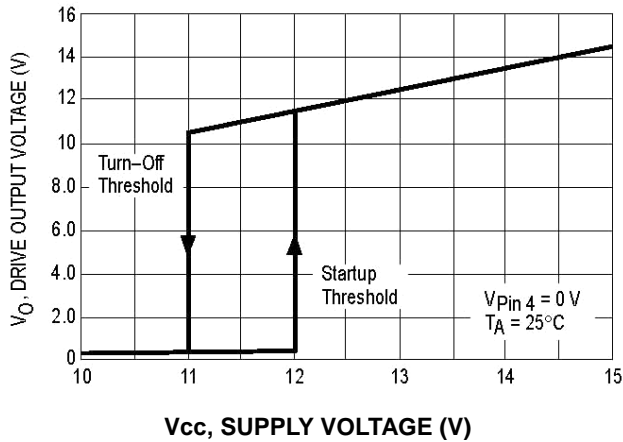
Figure 25. Drive Output Voltage Versus Supply Voltage
