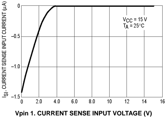
Figure 15. Current Sense Input Current Versus Voltage
