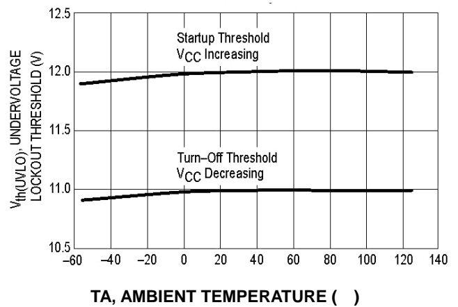
Figure 26. UVLO Thresholds Versus Temperature
