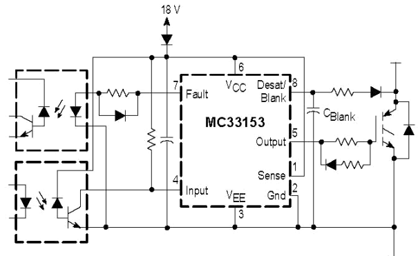
Figure 36. Desaturation Application
