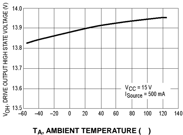
Figure 7. Drive Output High State Voltage Versus Temperature
