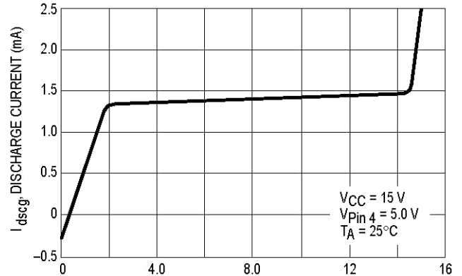
Figure 22. Fault Blanking/Desaturation Discharge Current versus Input Voltage
