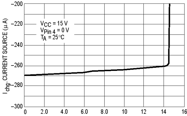
Figure 21. Fault Blanking/Desaturation Current Source Versus Input Voltage
