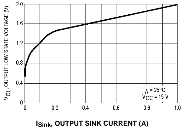
Figure 6. Drive Output Low State Voltage Versus Sink Current
