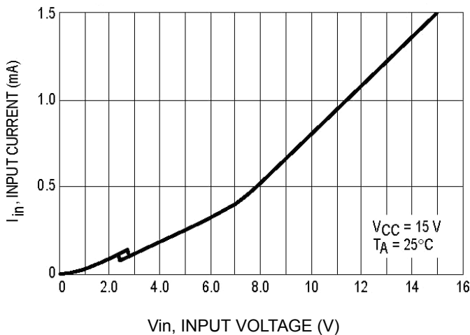
Figure 1. Input Current versus input voltage
