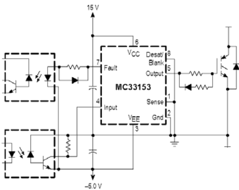
Figure 35. Dual Supply Application
