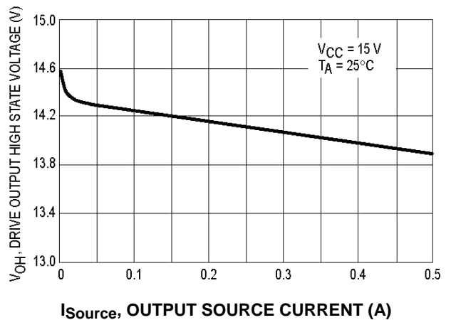
Figure 8. Drive Output High State Voltage Versus Source Current
