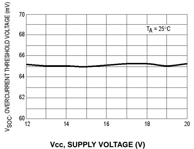
Figure 14. Short Circuit Comparator Threshold Voltage versus Supply Voltage
