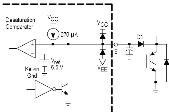
Figure 33.Desaturation Detection
