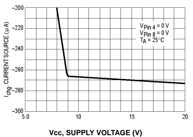
Figure 20. Fault Blanking/Desaturation Current Source versus Supply Voltage
