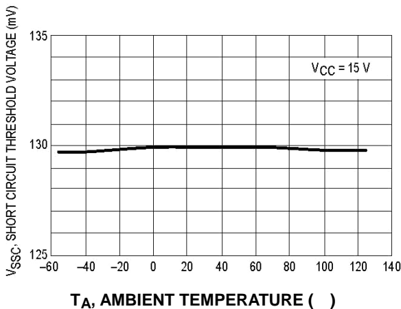
Figure 13. Short Circuit Comparator Threshold Voltage versus Temperature
