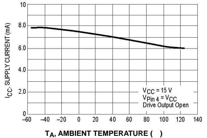
Figure 28. Supply Current versus Temperature
