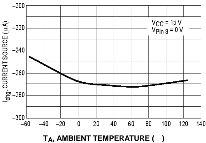
Figure 19. Fault Blanking/Desaturation Current Source versus Temperature
