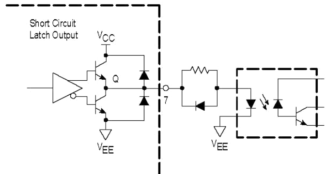
Figure 32. Output Fault Optoisolator
