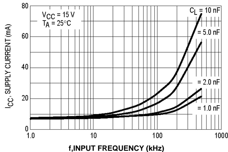
Figure 29. Supply Current versus Input Frequency
