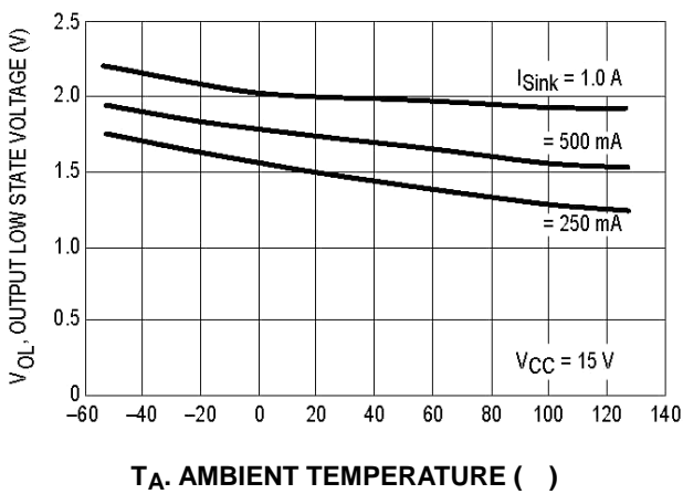
Figure 5. Drive Output Low State Voltage Versus Temperature
