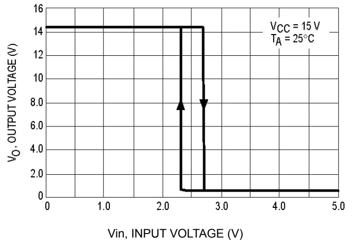
Figure 2. Output Voltage versus Input Voltage
