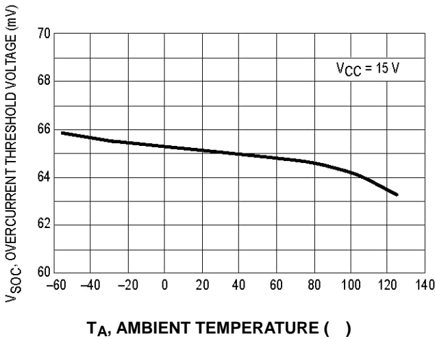
Figure 11. Overcurrent Protection Threshold Voltage versus Temperature
