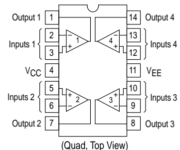
DTB SUFFIX PLASTIC PACKAGE CASE 948G (TSSOP-14)
