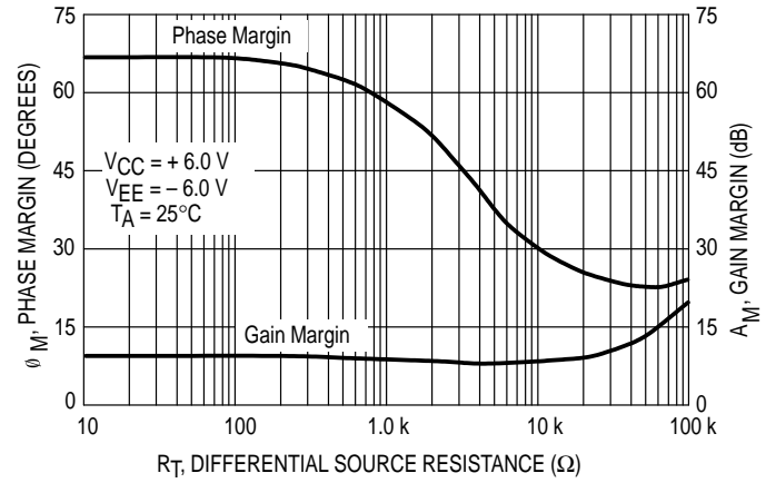
Figure 21. Gain and Phase Margin versus Differential Source Resistance
