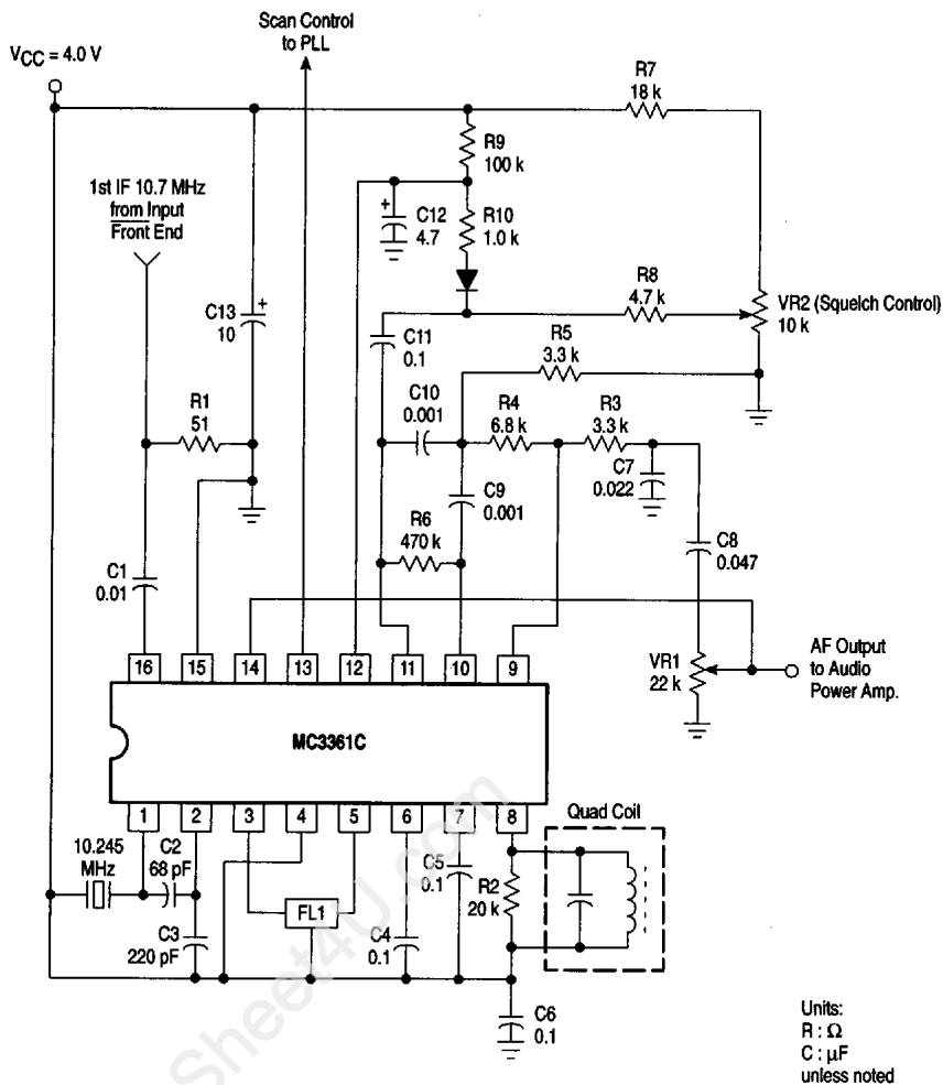
Figure 10. Simplified Application
