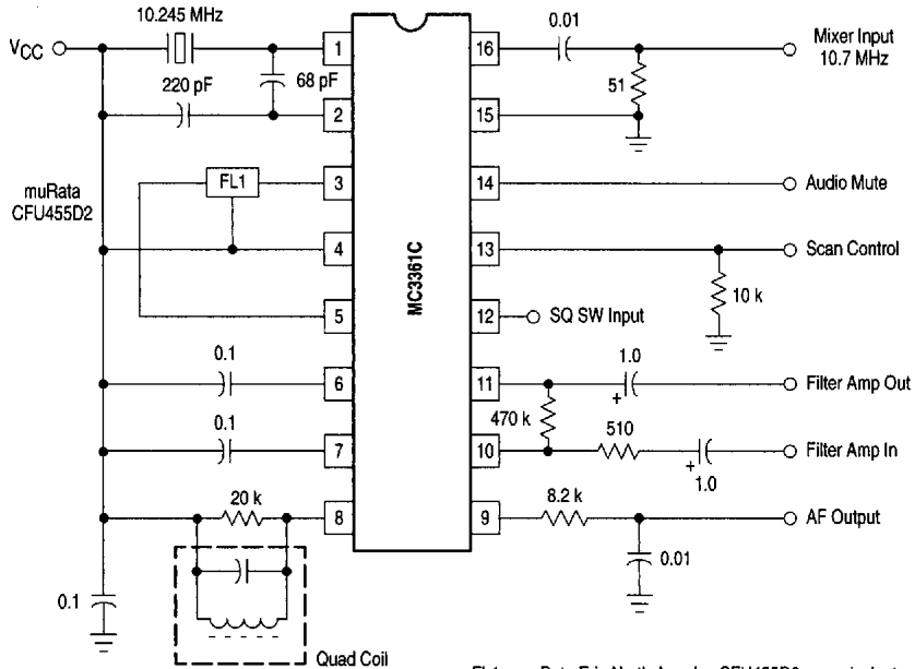
Figure 1. Test Circuit
