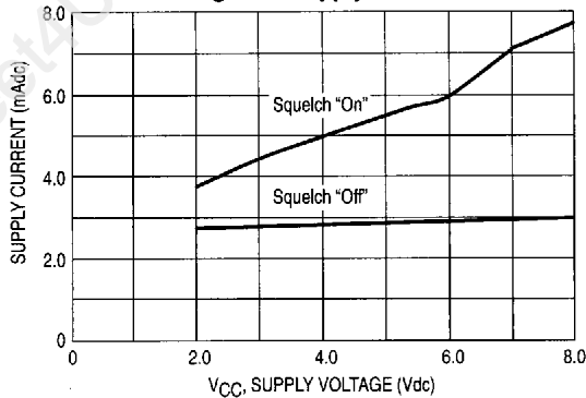
Figure 9. Supply Current
