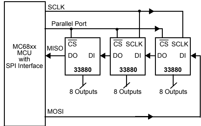
Figure 19. 33880 SPI System Daisy Chain
