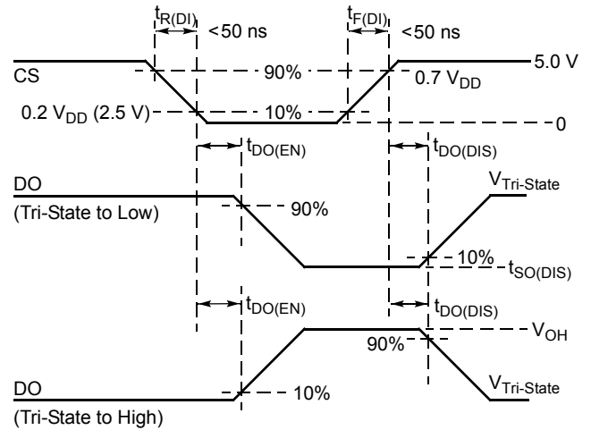
Figure 8. Turn-ON/OFF Waveforms
