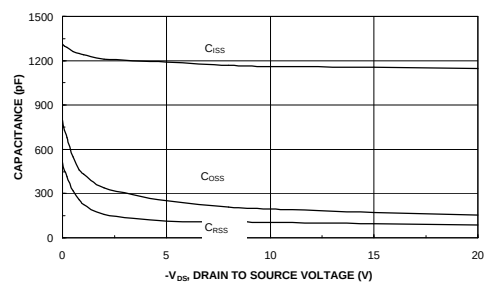
Figure 4. Capacitance
