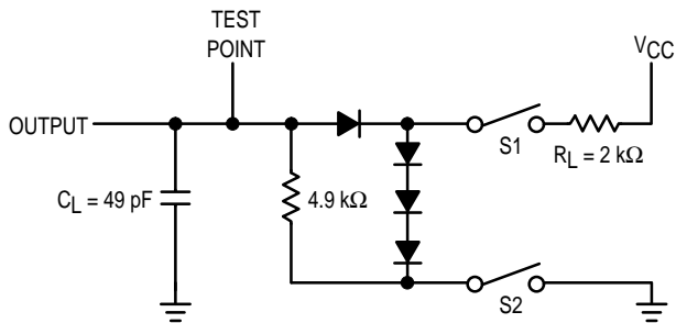
Figure 1. Test Circuit
