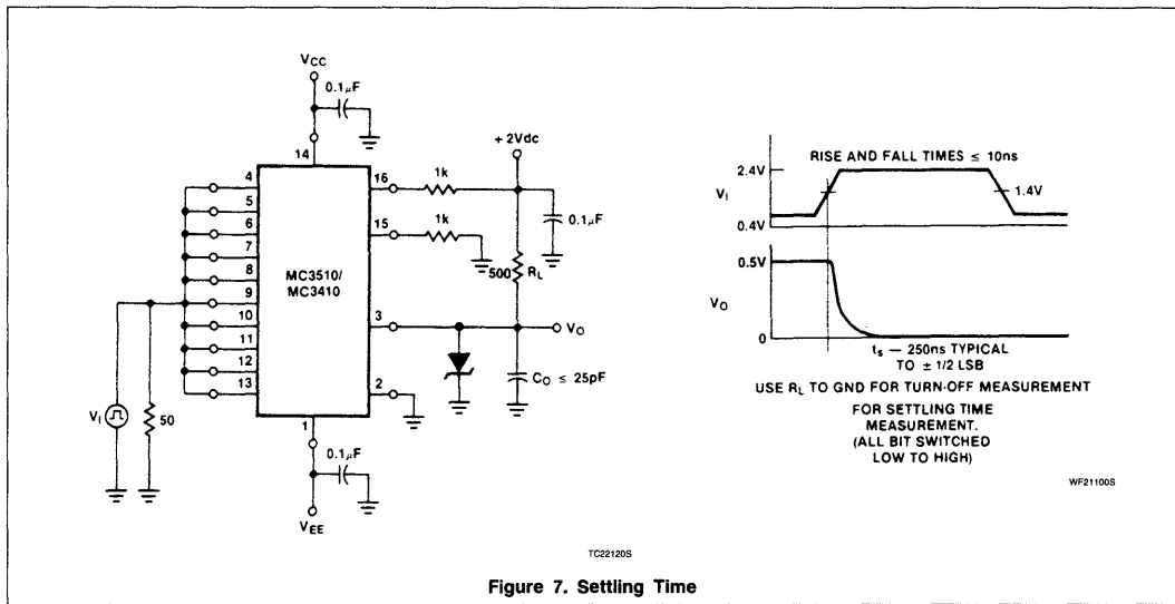
Figure 7. Settling Time
