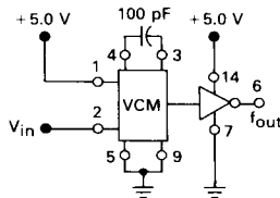
FIGURE 3 — VOLTAGE-CONTROLLED MULTIVIBRATOR
