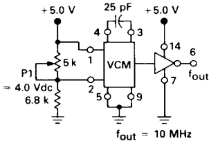
FIGURE 3 — VOLTAGE-CONTROLLED MULTIVIBRATOR
