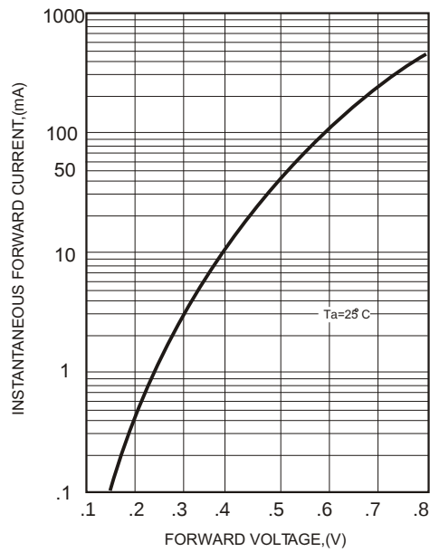
FIG.1-TYPICAL FORWARD CHARACTERISTICS
