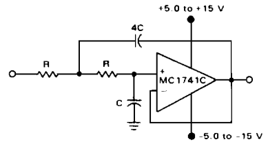
FIGURE 20 — OPERATIONAL AMPLIFIER LOW PASS FILTER
