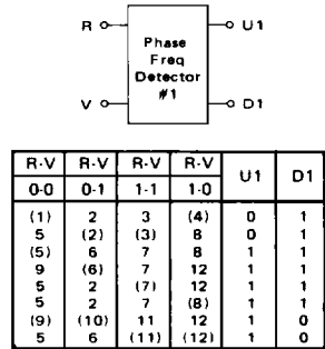
FIGURE 1 — PHASE DETECTOR #1 FLOW TABLE
