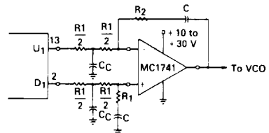
FIGURE 22 — TYPICAL FILTER AND SUMMING NETWORK
