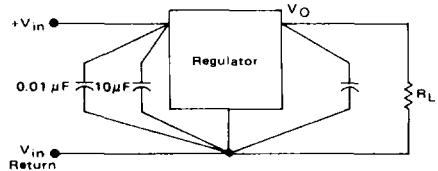
FIGURE 29 — SUGGESTED BYPASSING PROCEDURE
