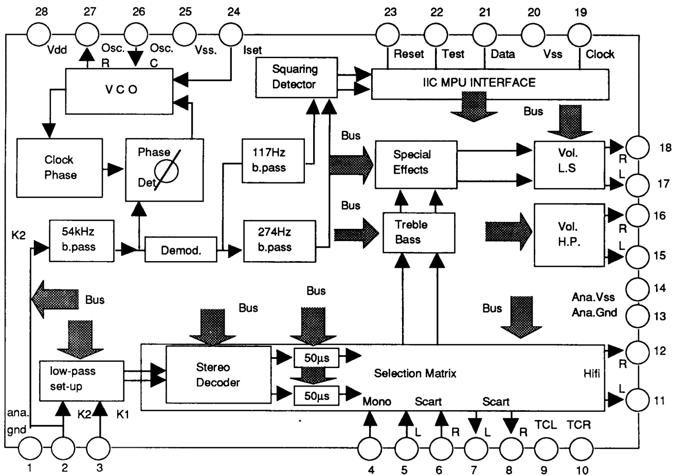
Figure 1. Block diagram
