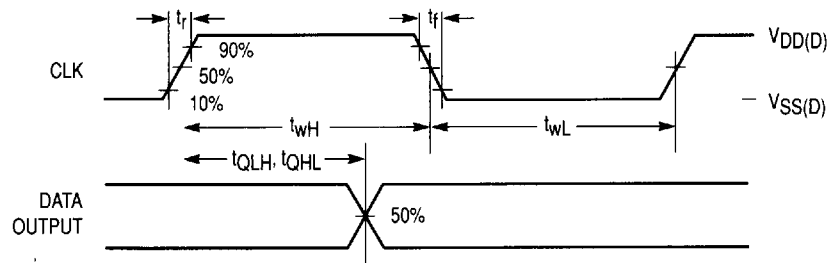
Figure 1. Clock and Output Timing
