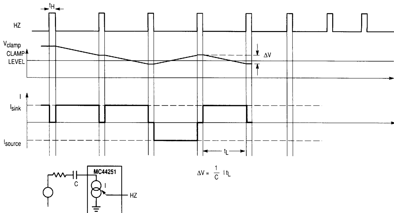
Figure 3. Clamp Network Timing Diagram — Operation
