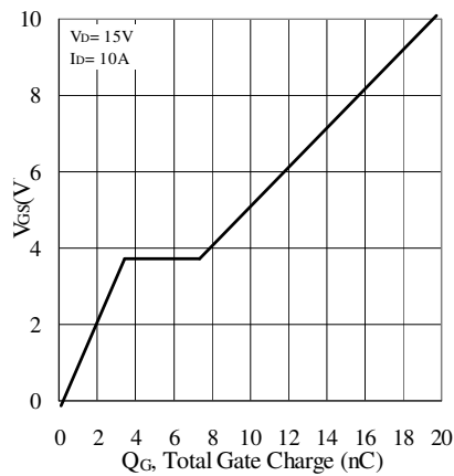
Gate Charge
