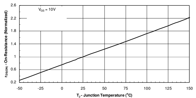
On-Resistance vs. Junction Temperature
