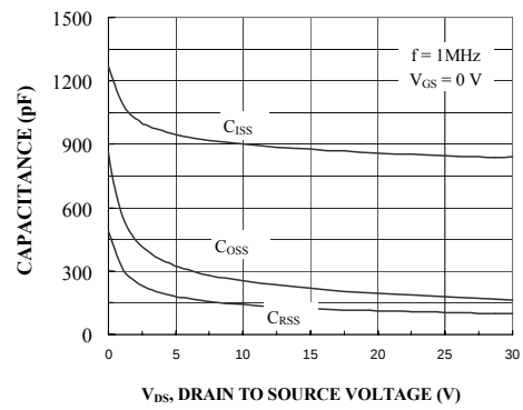
Figure 4. Capacitance Characteristics
