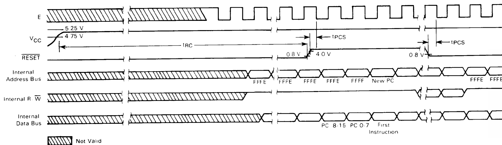
FIGURE 14 — RESET TIMING
