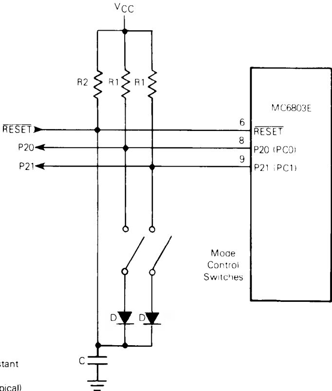
FIGURE 10 — TYPICAL MODE PROGRAMMING CIRCUIT
