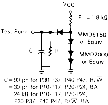
FIGURE 4 — TIMING TEST LOAD PORTS 1, 2, 3, 4
