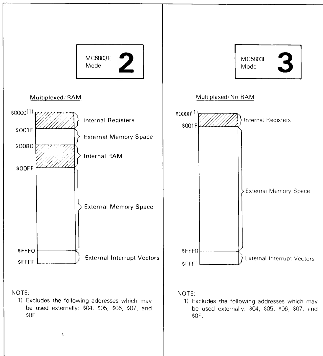
FIGURE 11 — MC6803E MEMORY MAPS
