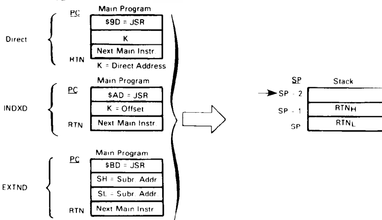
FIGURE 21 — SPECIAL OPERATIONS
