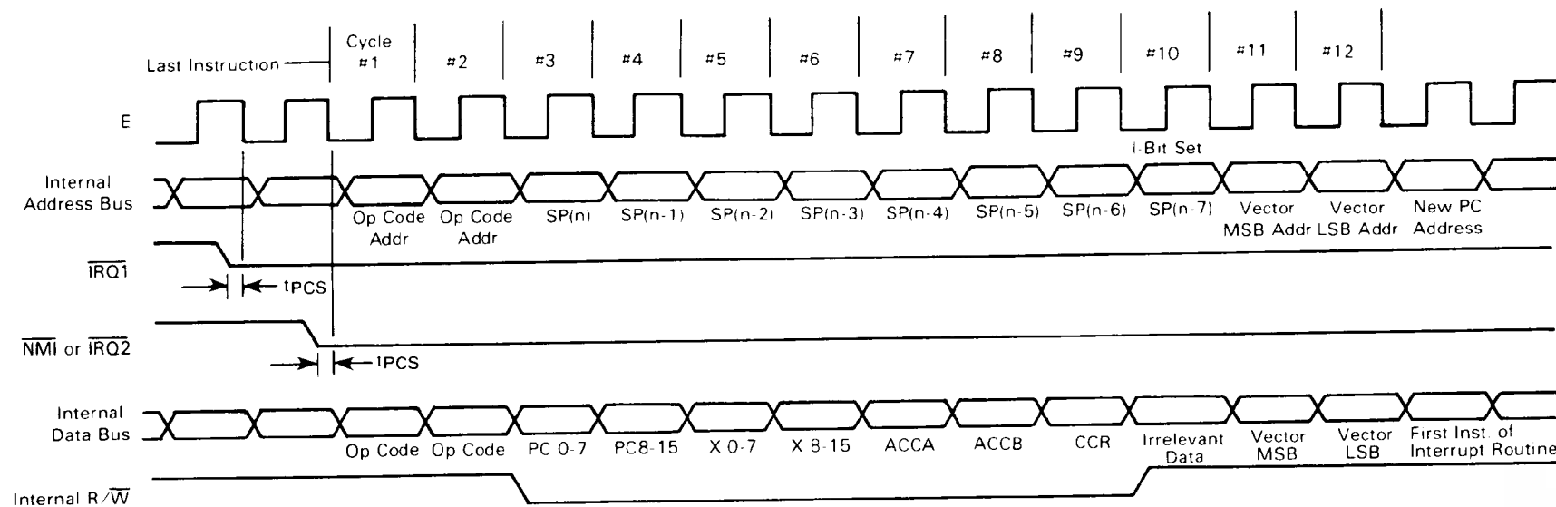
FIGURE 13 — INTERRUPT SEQUENCE
