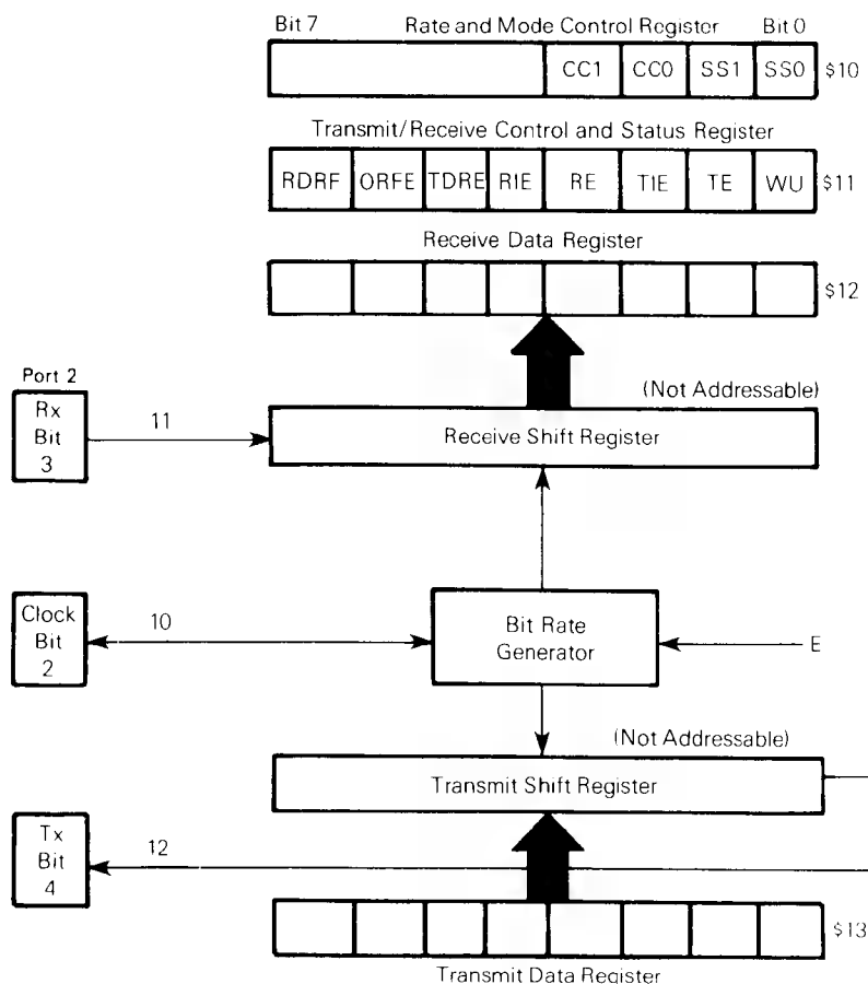
FIGURE 19 — SCI REGISTERS
