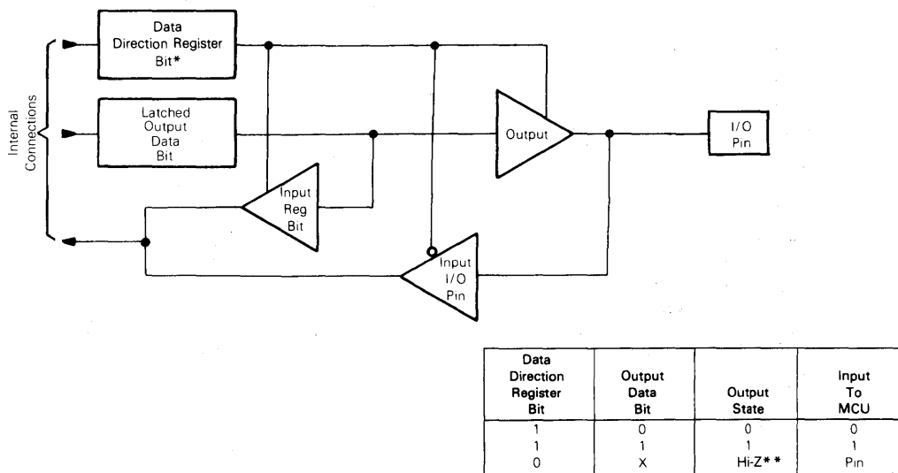
FIGURE 18 — TYPICAL PORT I/O CIRCUITRY
