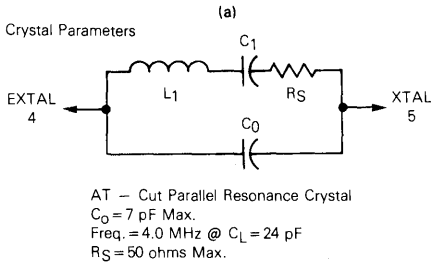
FIGURE 14 — CRYSTAL MOTIONAL ARM PARAMETERS AND SUGGESTED PC BOARD LAYOUT
