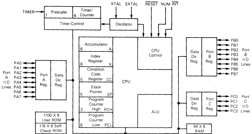
FIGURE 1 — MC6805P2 HMOS MICROCOMPUTER BLOCK DIAGRAM
