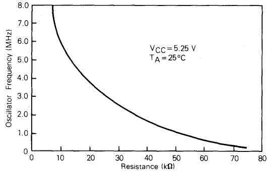
FIGURE 15 — TYPICAL FREQUENCY SELECTION FOR RESISTOR OSCILLATOR OPTION
