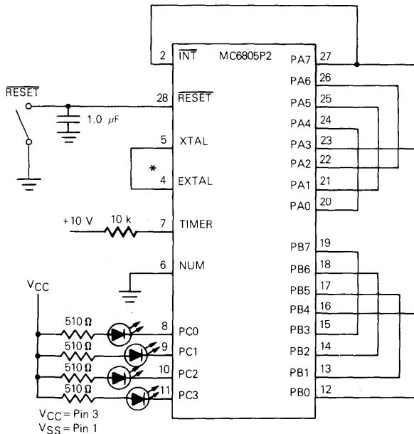
FIGURE 9 — SELF-CHECK CONNECTIONS
