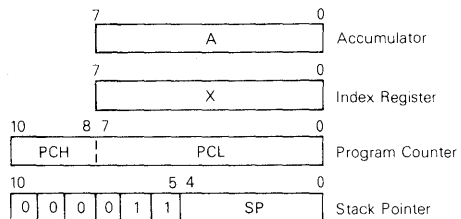
FIGURE 7 — PROGRAMMING MODEL
