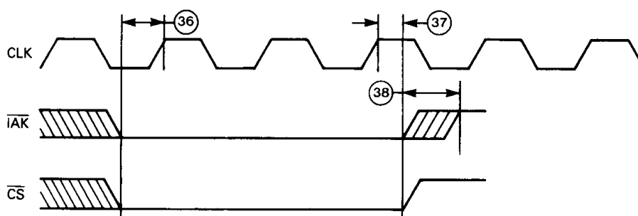
FIGURE 13 — RESET
