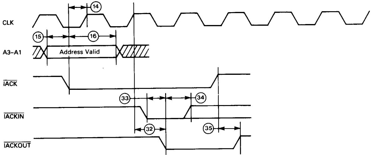
FIGURE 12 — INTERRUPT ACKNOWLEDGE CYCLE — IACKOUT
