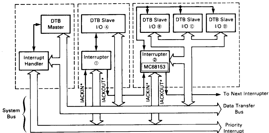
FIGURE 5 — SIMPLE VMEbus CONFIGURATION
