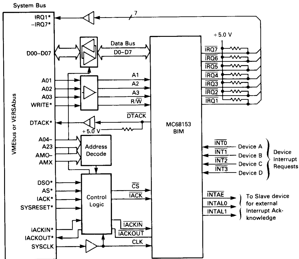
FIGURE 7 — VMEbus/VERSAbus INTERFACE BLOCK DIAGRAM
