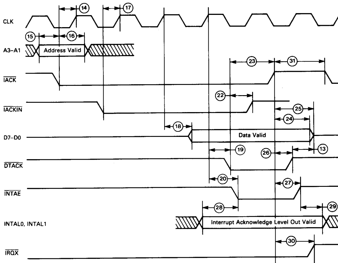
FIGURE 10 — INTERRUPT ACKNOWLEDGE CYCLE — INTERNAL VECTOR
