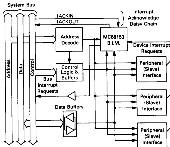
FIGURE 1 — BLOCK DIAGRAM
