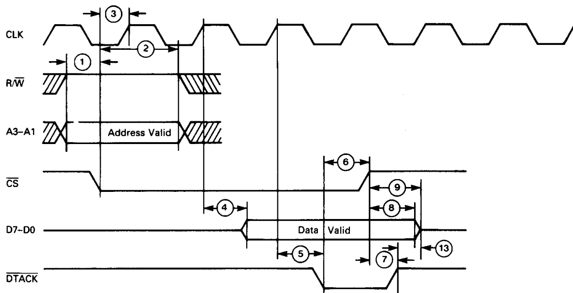
FIGURE 8 — READ CYCLE
