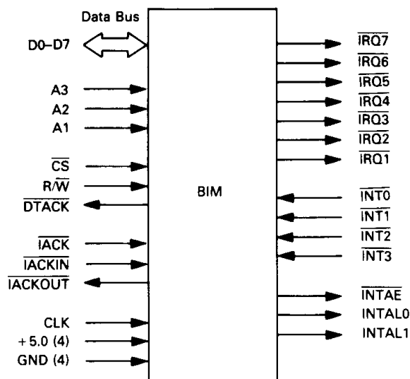
FIGURE 3 — LOGICAL PIN ASSIGNMENT
