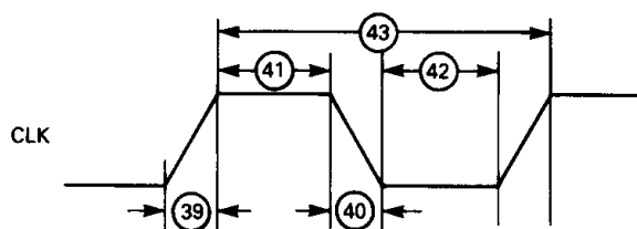
FIGURE 14 — CLOCK WAVEFORM
