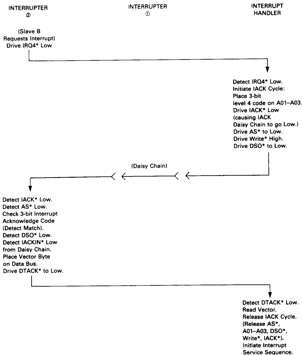
FIGURE 6 — INTERRUPT REQUEST AND ACKNOWLEDGE OPERATION FLOW DIAGRAM
