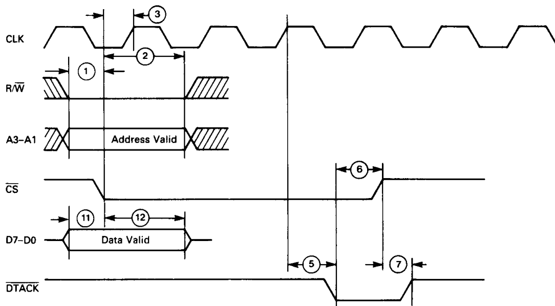
FIGURE 9 — WRITE CYCLE
