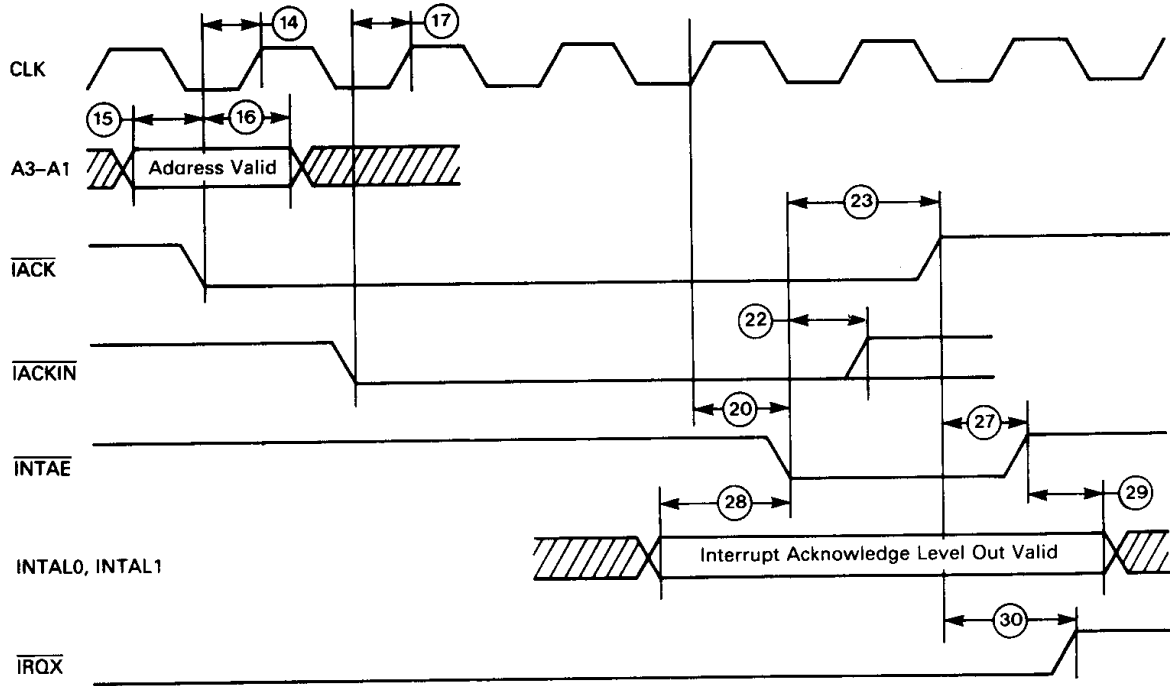
FIGURE 11 — INTERRUPT ACKNOWLEDGE CYCLE — EXTERNAL VECTOR
