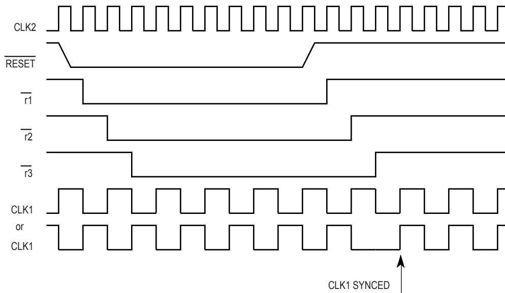
Figure 2-2. CLK1 Phase Relationship
