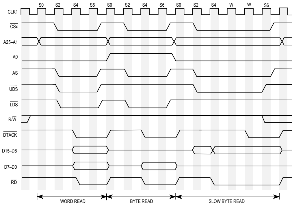
Figure 4-3. External Timing Diagram to Chip-Select Banks
