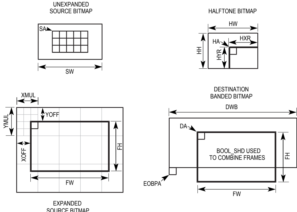
Figure 13-11. Expanded Source, Halftone, Destination bitBLT To Banded Bitmap, 0° Page
