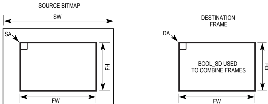
Figure 13-14. Source/Destination bitBLT to Frame
