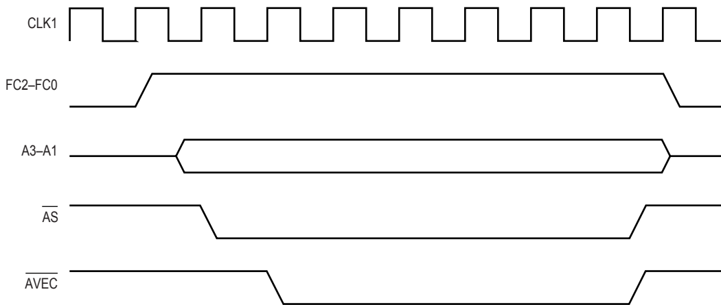
Figure 4-8. Internal Interrupt Acknowledge Cycle
