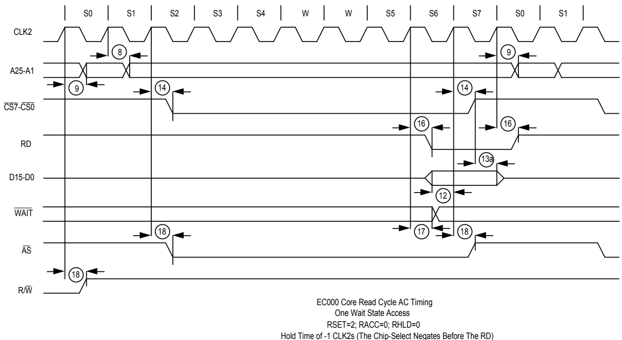
Figure 14-11. Read Access (6:2:-1:3)
