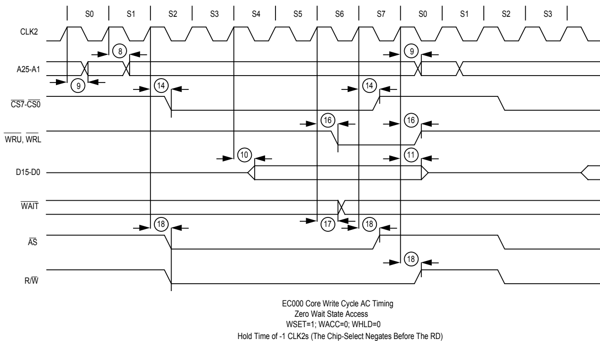
Figure 14-12. Write Access (4:2:-1:3)
