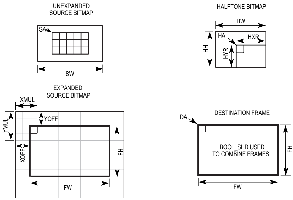
Figure 13-17. Expanded Source, Halftone, Destination bitBLT To Frame
