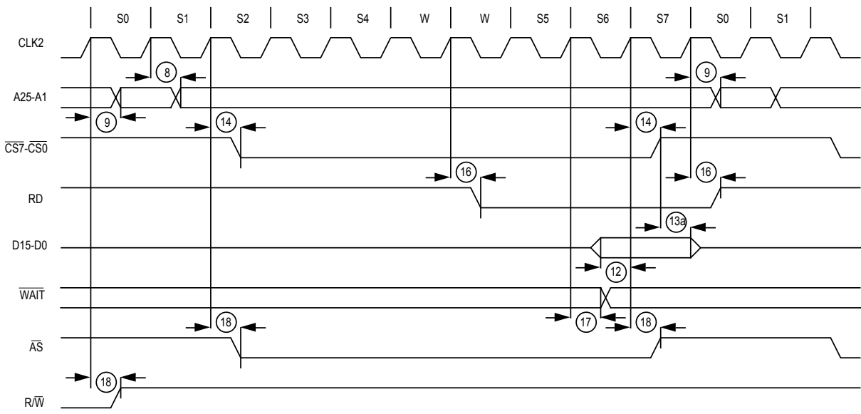
EC000 Core Read Cycle AC Timing One Wait State Access RSET=1; RACC=1; RHLD=0 Hold Time of -1 CLK2s (The Chip-Select Negates Before The RD)
