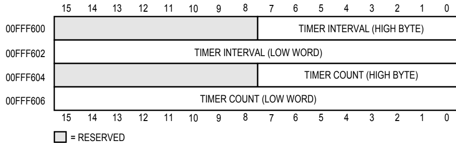
Figure 5-3. Timer Register
