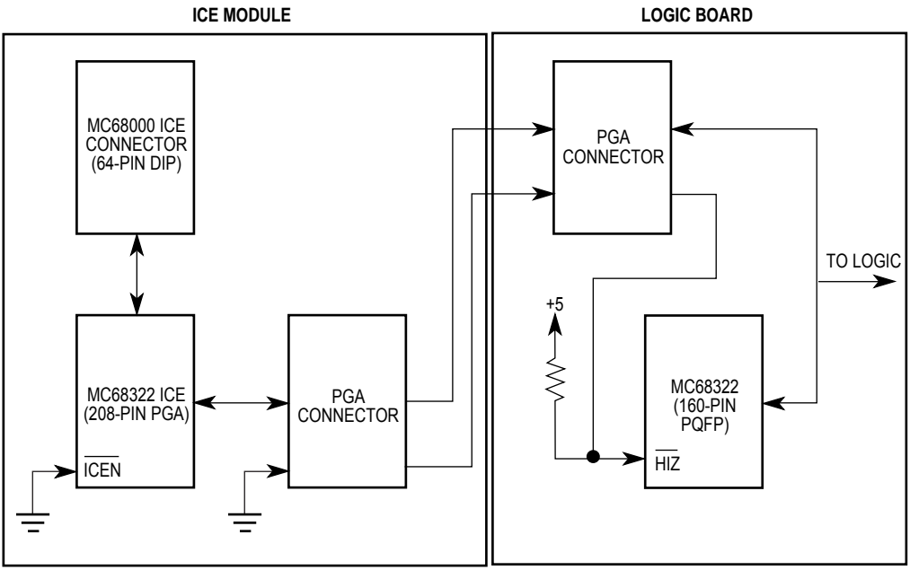
Figure A-1. ICE Interface Block Diagram
