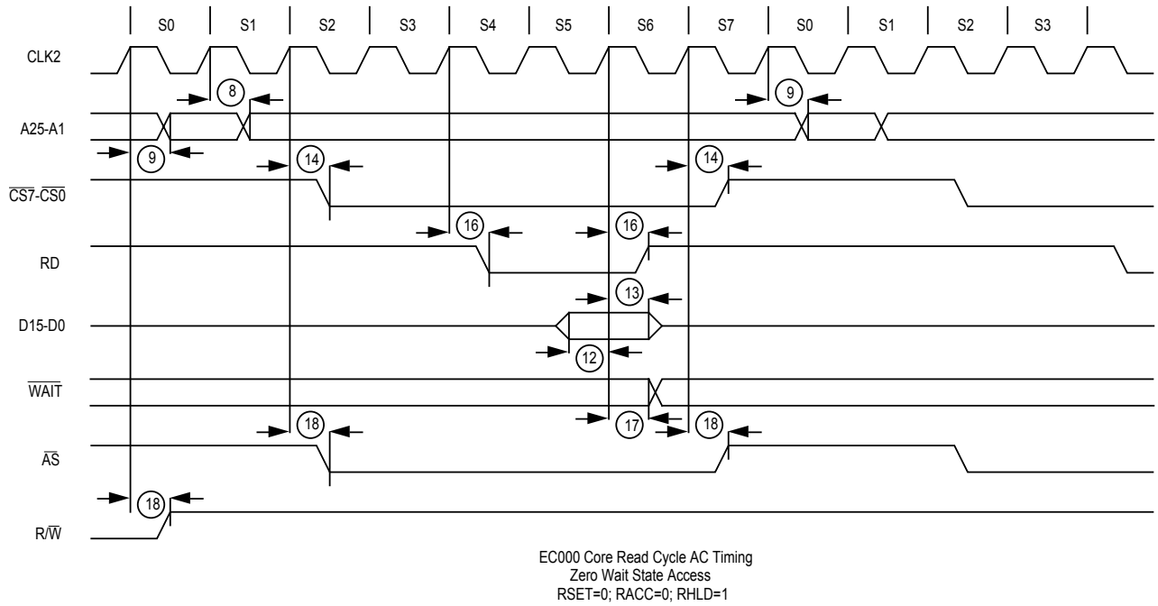
Figure 14-3. Read Access (2:2:1:3)
