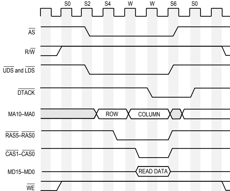
Figure 4-3. External Timing Diagram to Chip-Select Banks
