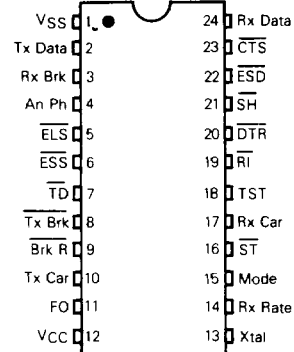
PIN ASSIGNMENT
