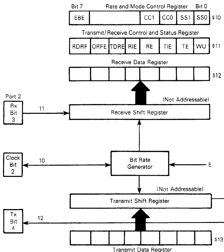
FIGURE 22 — SCI REGISTERS
