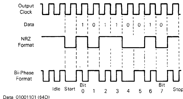
FIGURE 23 — SCI DATA FORMATS
