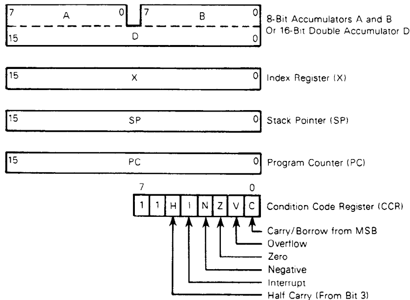
FIGURE 8 — PROGRAMMING MODEL
