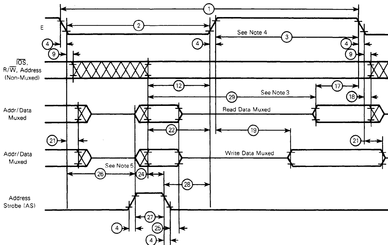
FIGURE 7 — BUS TIMING
