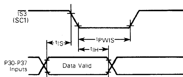
FIGURE 4 — PORT 3 LATCH TIMING (SINGLE-CHIP MODE)
