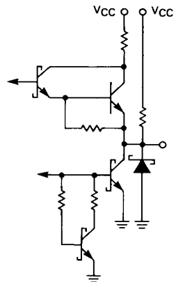
FIGURE 22 — TYPICAL INPUT
