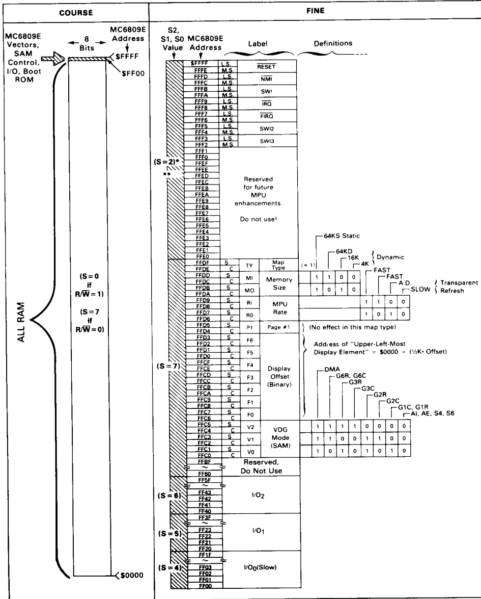
FIGURE 16 — LS785 MEMORY MAP (TYPE #1 64K RAM)
