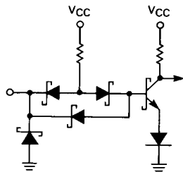
FIGURE 23 — TYPICAL OUTPUT
