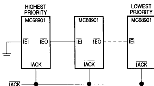
Figure 3. Daisy-Chain Interrupt Structure
