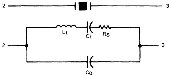
Equivalent Circuit
