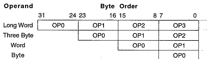
Figure 3–8. Operand Byte Order
