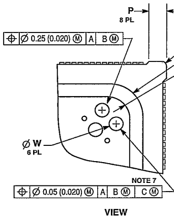
CASE 887-01 ISSUE 0
