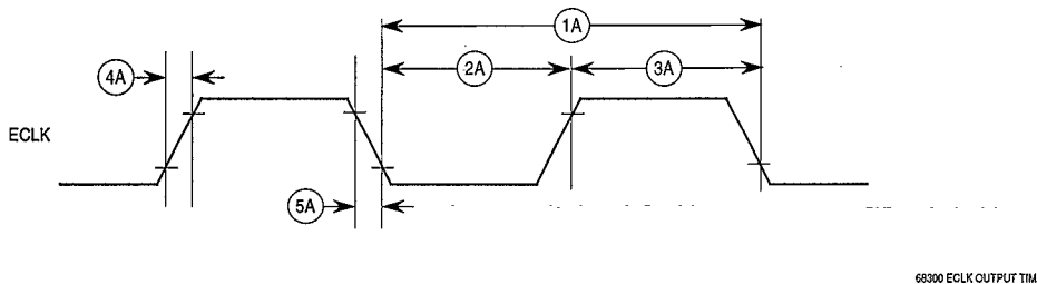
Figure A-3. ECLK Output Timing Diagram
