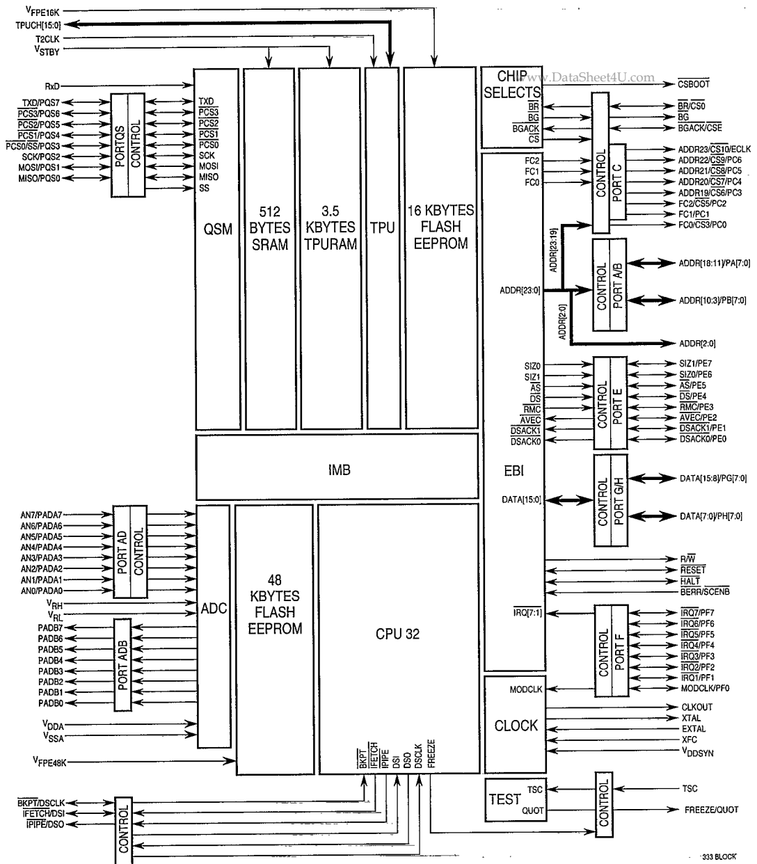
Figure 1-1. MC68F333 Block Diagram
