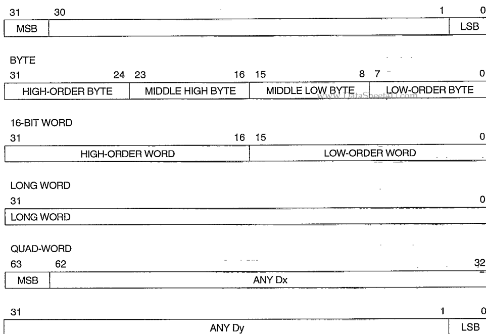
Figure 4-4. Data Organization in Data Registers
