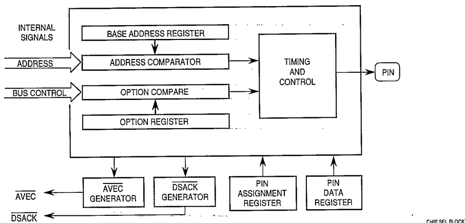
Figure 3–19. Chip-Select Circuit Block Diagram
