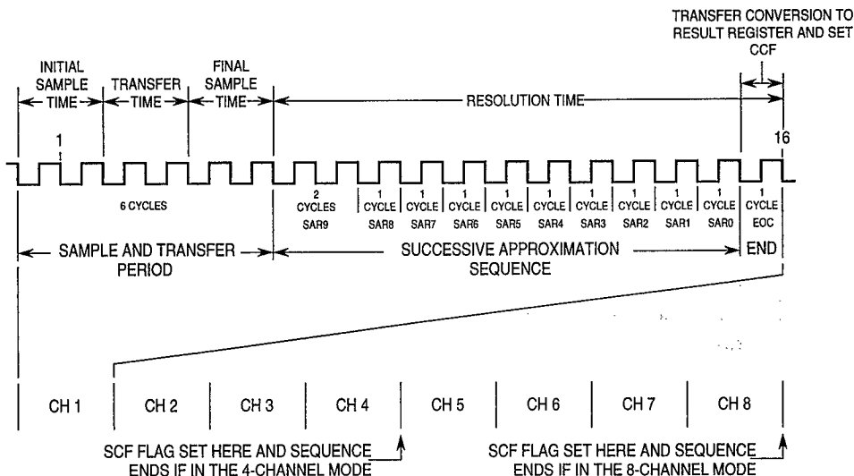
Figure 7-2. 8-Bit Conversion Timing
