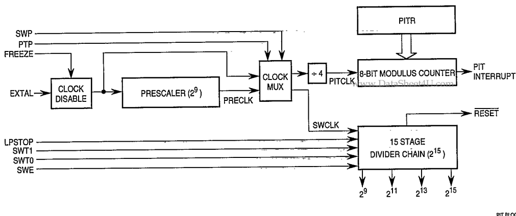
Figure 3–3. Periodic Interrupt Timer and Software Watchdog Timer
