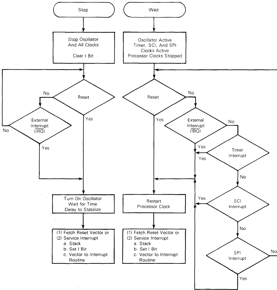
Figure 3-3. STOP/WAIT Flowcharts
