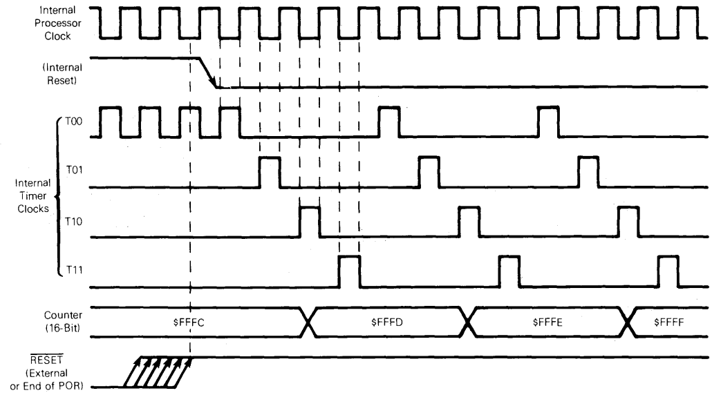
Figure 4-2. Timer State Timing Diagram For Reset
