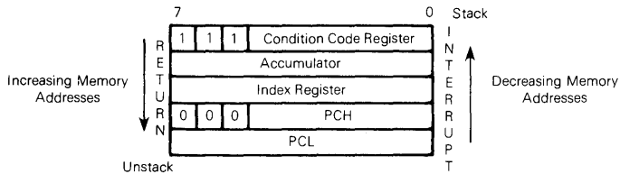
Figure 2-5. Programming Model
