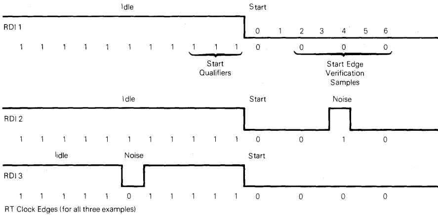
Figure 5-2. Examples of Start Bit Sampling Technique
