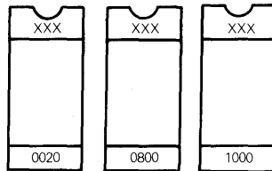
Figure 10-1. EPROM Marking Example
