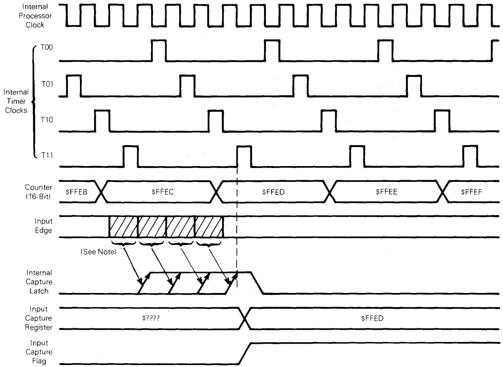
Figure 4-3. Timer State Timing Diagram For Input Capture
