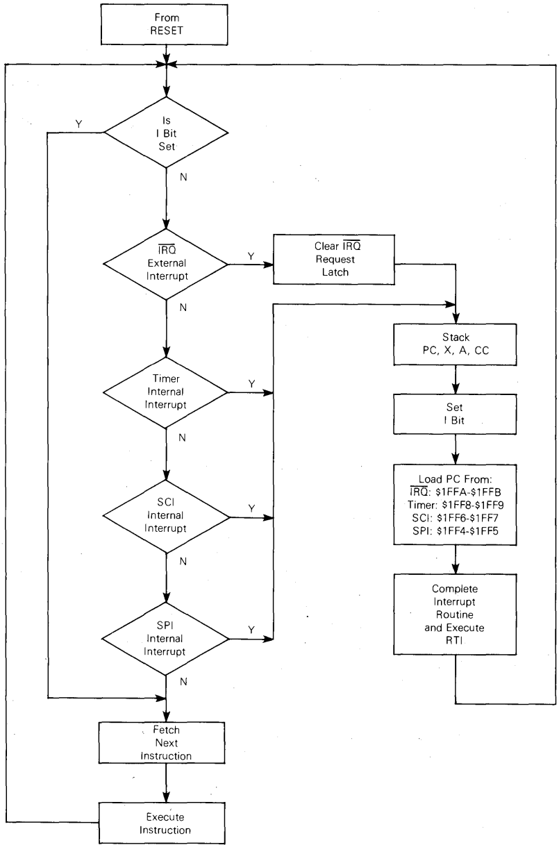
Figure 3-2. Hardware Interrupt Flowchart
