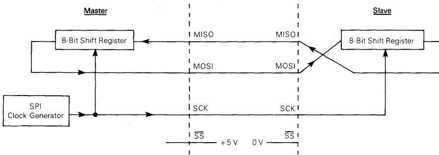
Figure 6-4. Serial Peripheral Interface Master-Slave Interconnection
