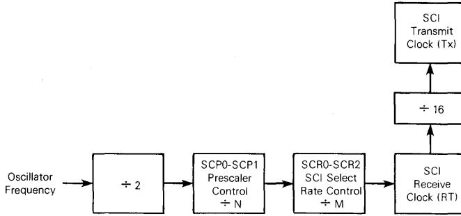
Figure 5-7. Rate Generator Division
