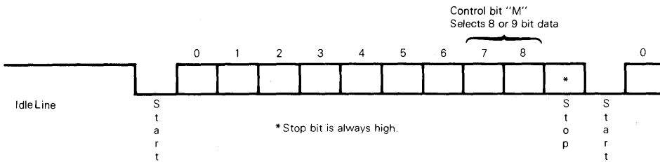
Figure 5-1. Data Format
