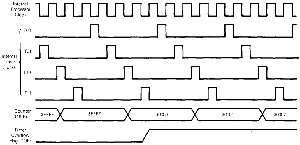
Figure 4-5. Timer State Diagram For Timer Overflow
