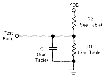
Figure 9-1. Equivalent Test Load
