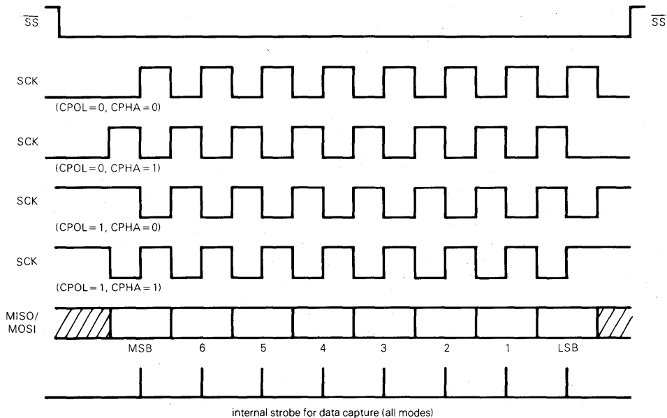
Figure 6-2. Data Clock Timing Diagram
