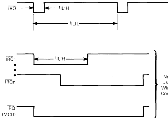
(b) Interrupt Mode Diagram
