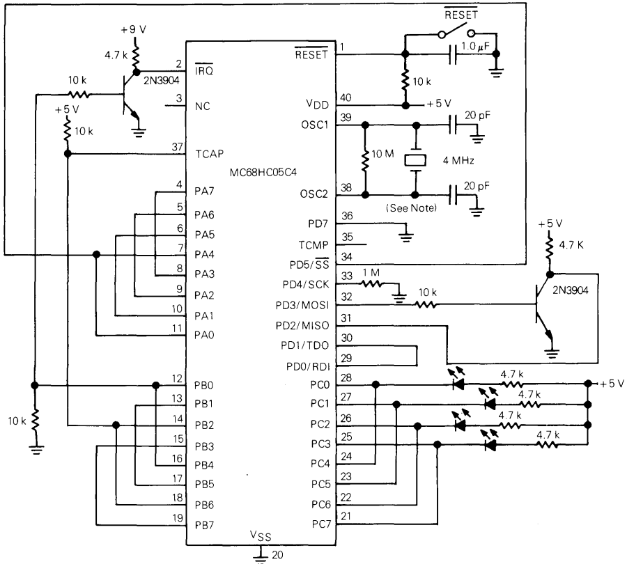
Figure 2-7. Self-Check Circuit Schematic Diagram
