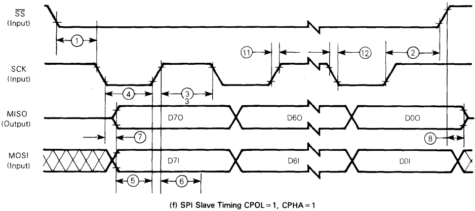
Figure 9-5. Timing Diagrams (Continued)
