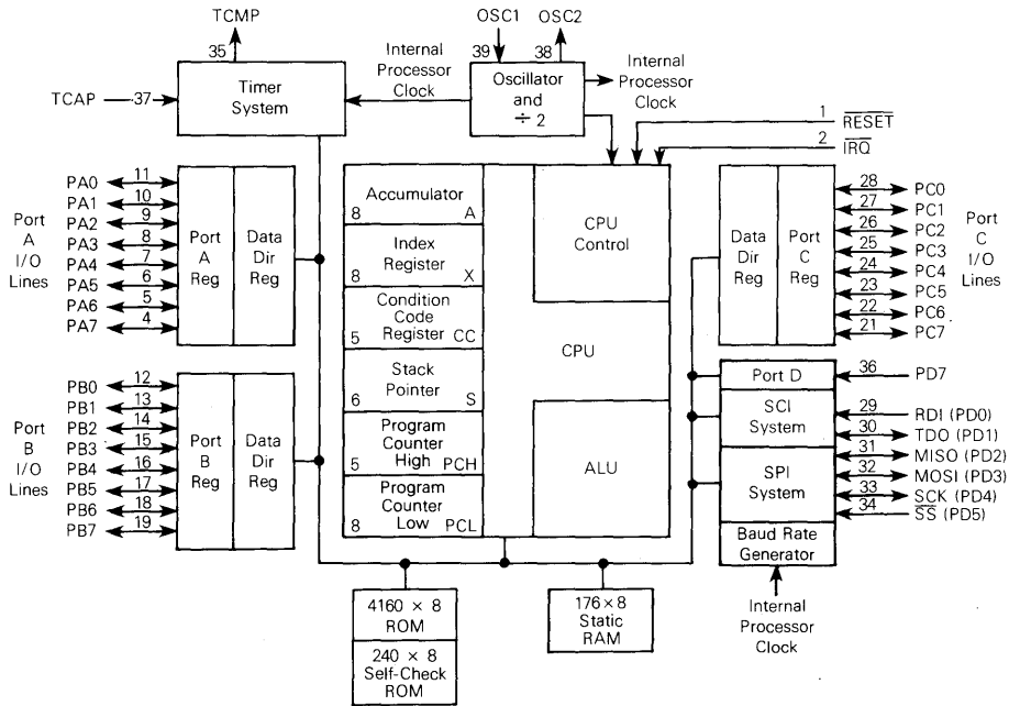
Figure 1-1. MC68HC05C4 Microcomputer Block Diagram
