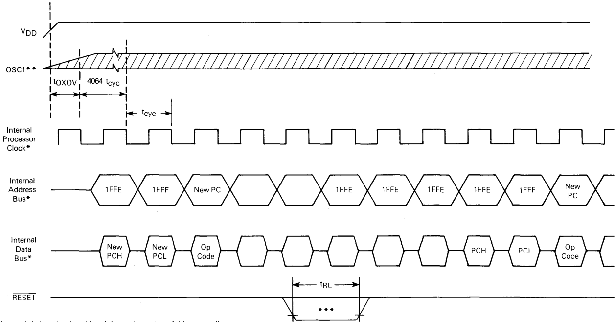
Figure 3-1. Power-On Reset and RESET
