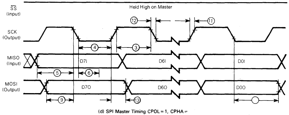
Figure 9-5. Timing Diagrams (Continued)
