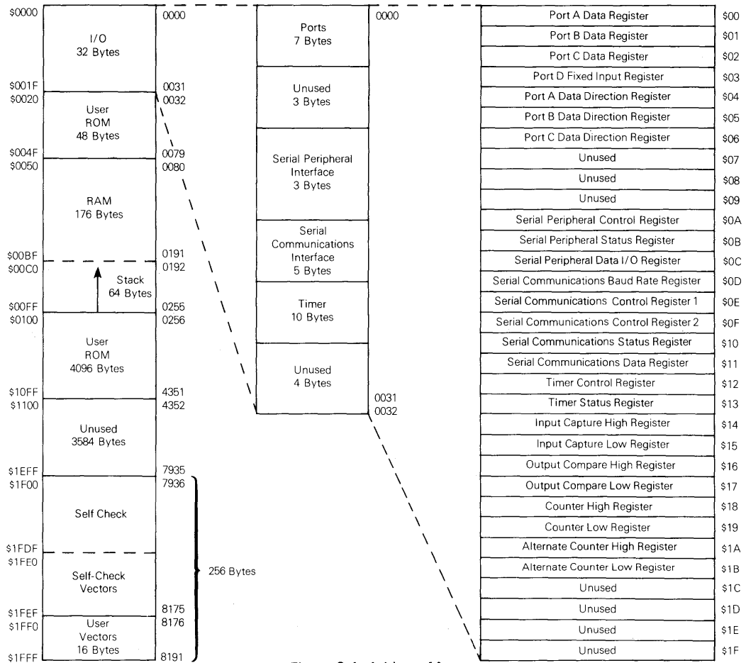
Figure 2-4. Address Map
