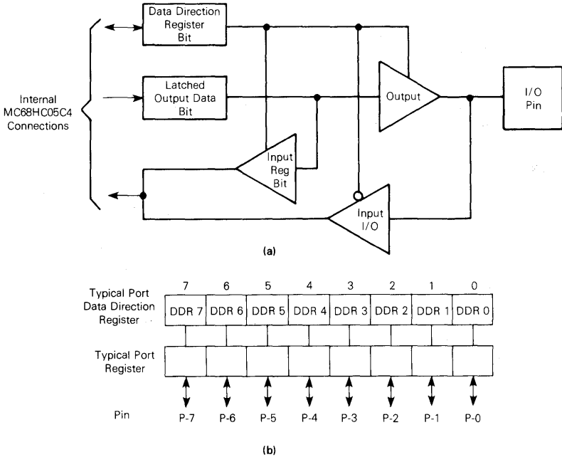
Figure 2-3. Typical Parallel Port I/O Circuitry
