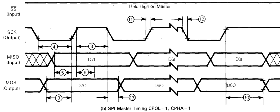
Figure 9-5. Timing Diagrams
