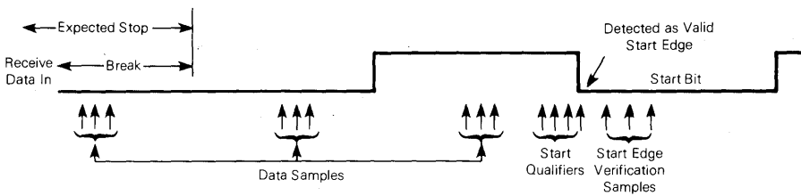
Figure 5-5. SCI Start Bit Following A Break
