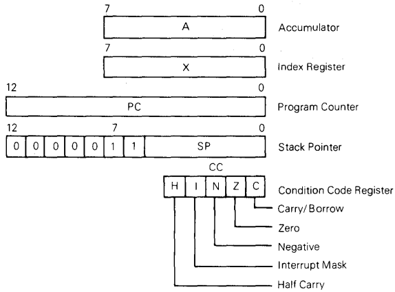
Figure 2-5. Programming Model
