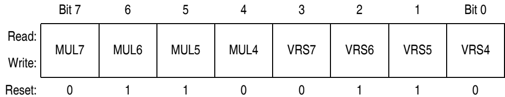
Figure 8-5. PLL Programming Register (PPG)
