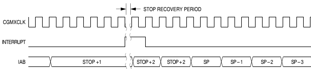
Figure 14-17. Stop Mode Recovery from Interrupt
