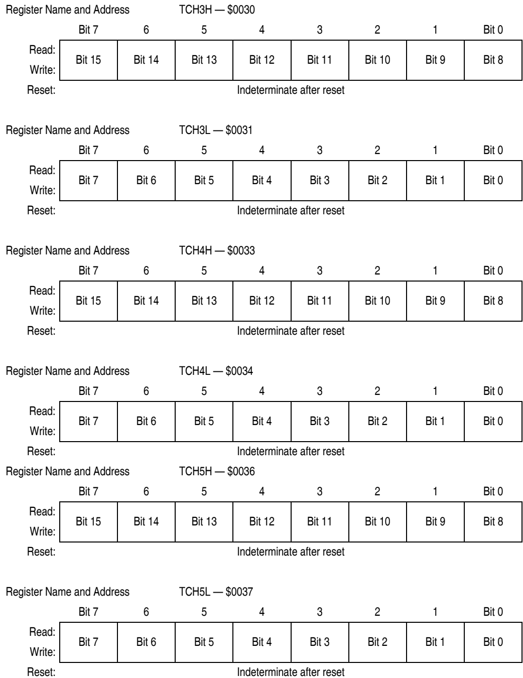
Figure 16-10. TIM Channel Registers (TCH0H/L–TCH3H/L) (Continued)
