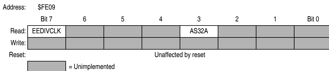
Figure 10-2. Mask Option Register 2 (MORB)
