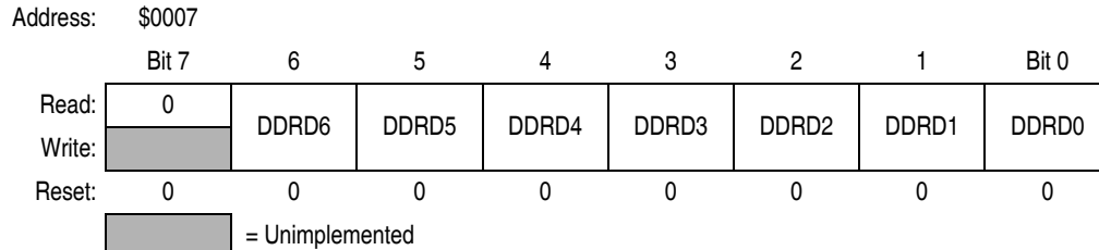
Figure 12-12. Data Direction Register D (DDRD)
