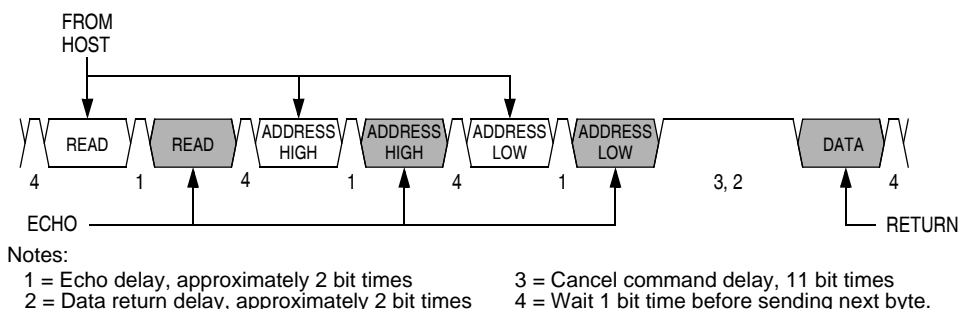
Figure 17-10. Read Transaction
