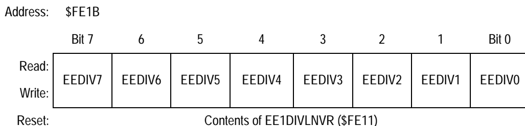
Figure 5-6. EE1DIV Divider Low Register (EE1DIVL)
