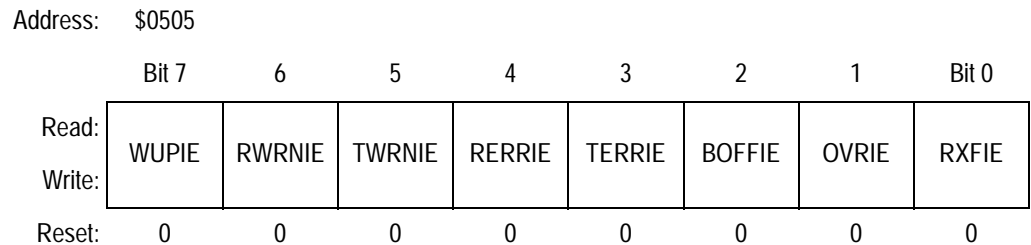
Figure 21-20. Receiver Interrupt Enable Register (CRIER)
