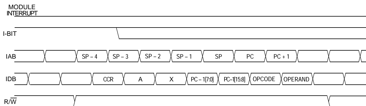
Figure 8-8. Interrupt Recovery
