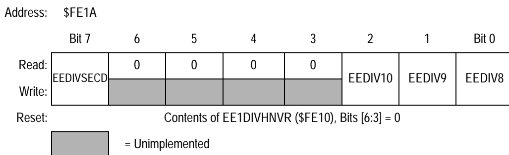
Figure 5-5. EE1DIV Divider High Register (EE1DIVH)
