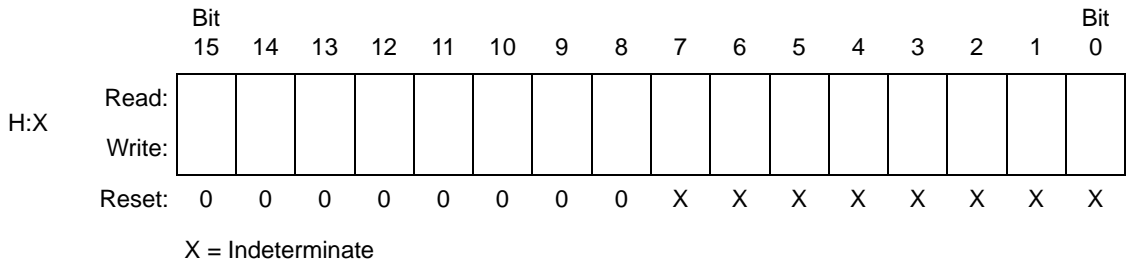
Figure 7-3. Index Register (H:X)
