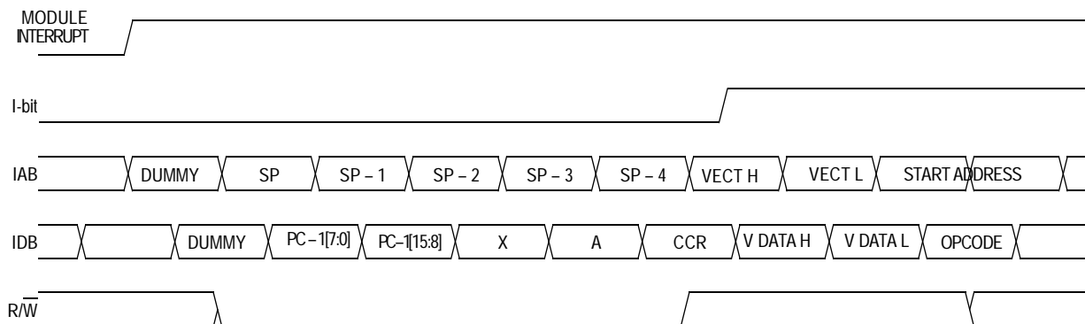
Figure 8-7. Interrupt Entry
