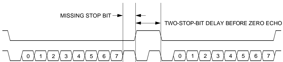
Figure 12-5. Break Transaction
