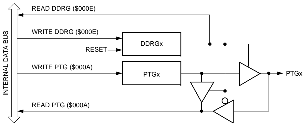
Figure 20-21. Port G I/O Circuit
