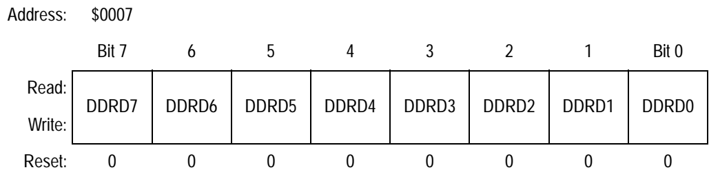
Figure 12. Data Direction Register D (DDRD)
