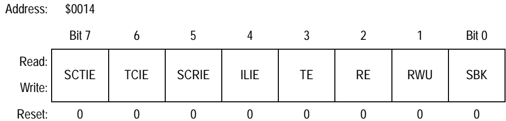
Figure 12. SCI Control Register 2 (SCC2)
