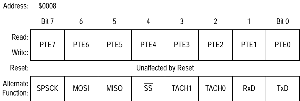
Figure 14. Port E Data Register (PTE)
