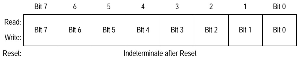
Figure 9. TIMB Channel Registers (TBCH0H/L–TBCH1H/L)
