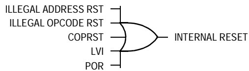
Figure 6. Sources of Internal Reset
