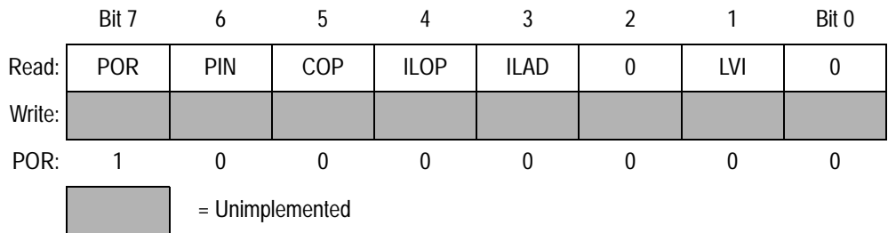
Figure 18. SIM Reset Status Register (SRSR)
