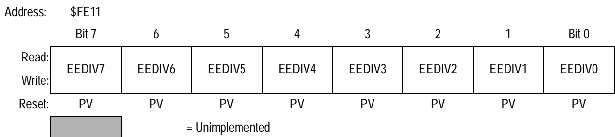
Figure 6. EEPROM-2 Divider Low Non-volatile Register (EEDIVLNVR)
