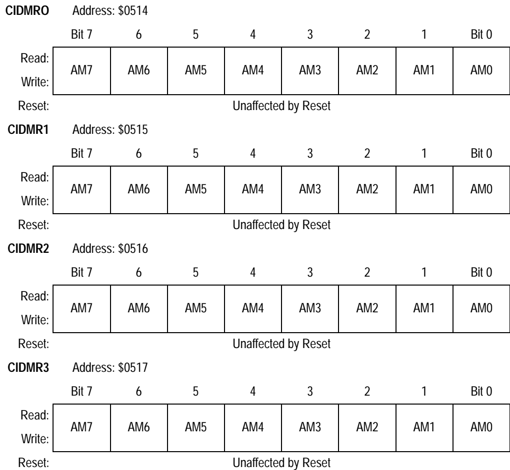
Figure 27. Identifier Mask Registers (CIDMR0–CIDMR3)
