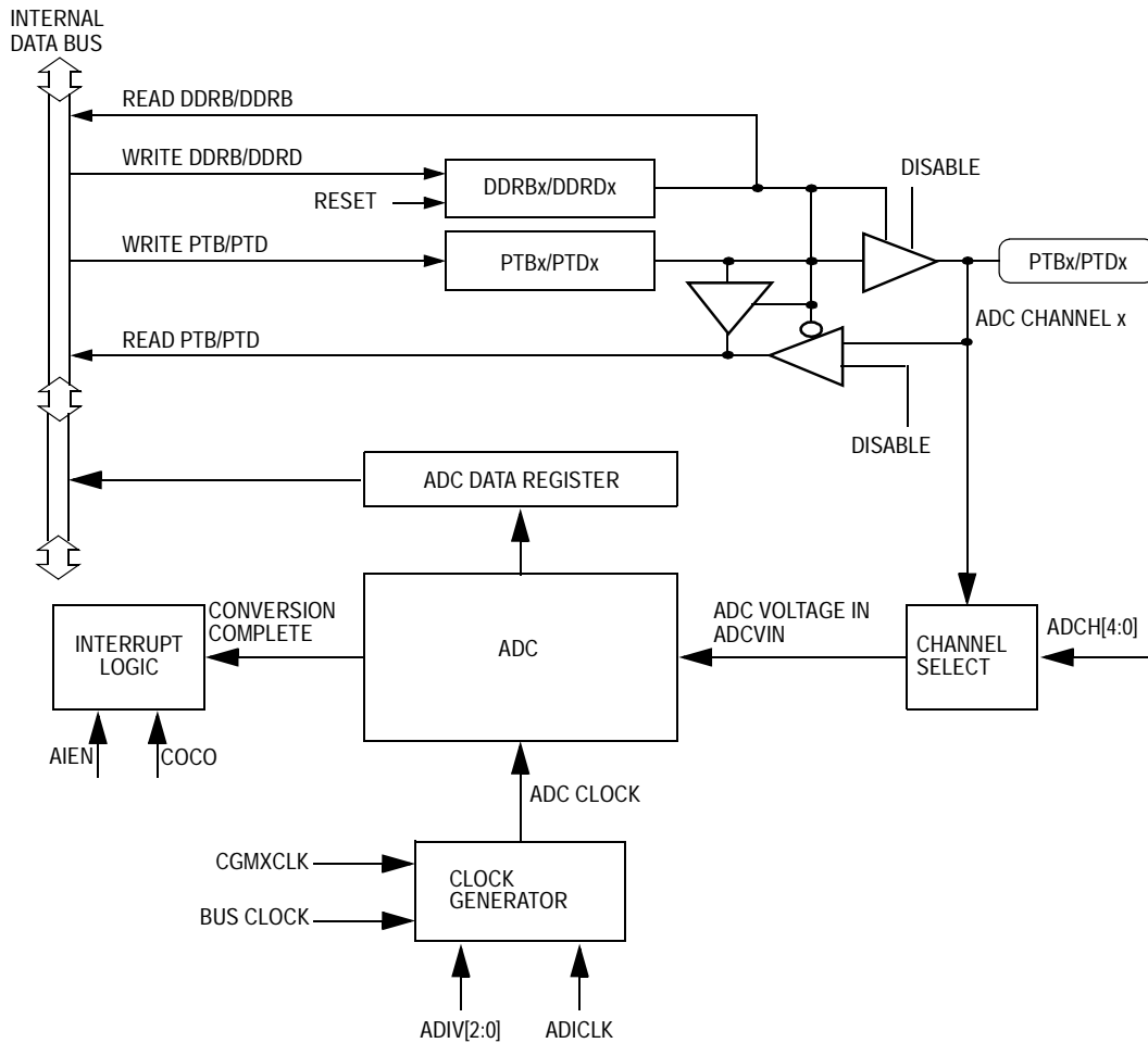
Figure 1. ADC Block Diagram
