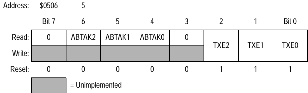
Figure 21. Transmitter Flag Register (CTFLG)
