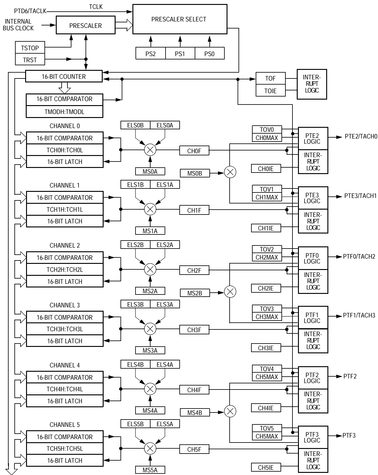
Figure 1. TIMA Block Diagram
