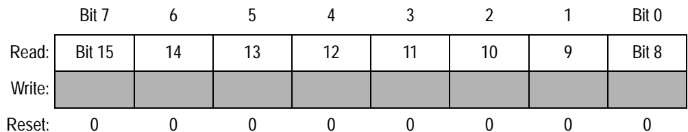
Figure 4. TIM Counter Registers (TCNTH–TCNTL)
