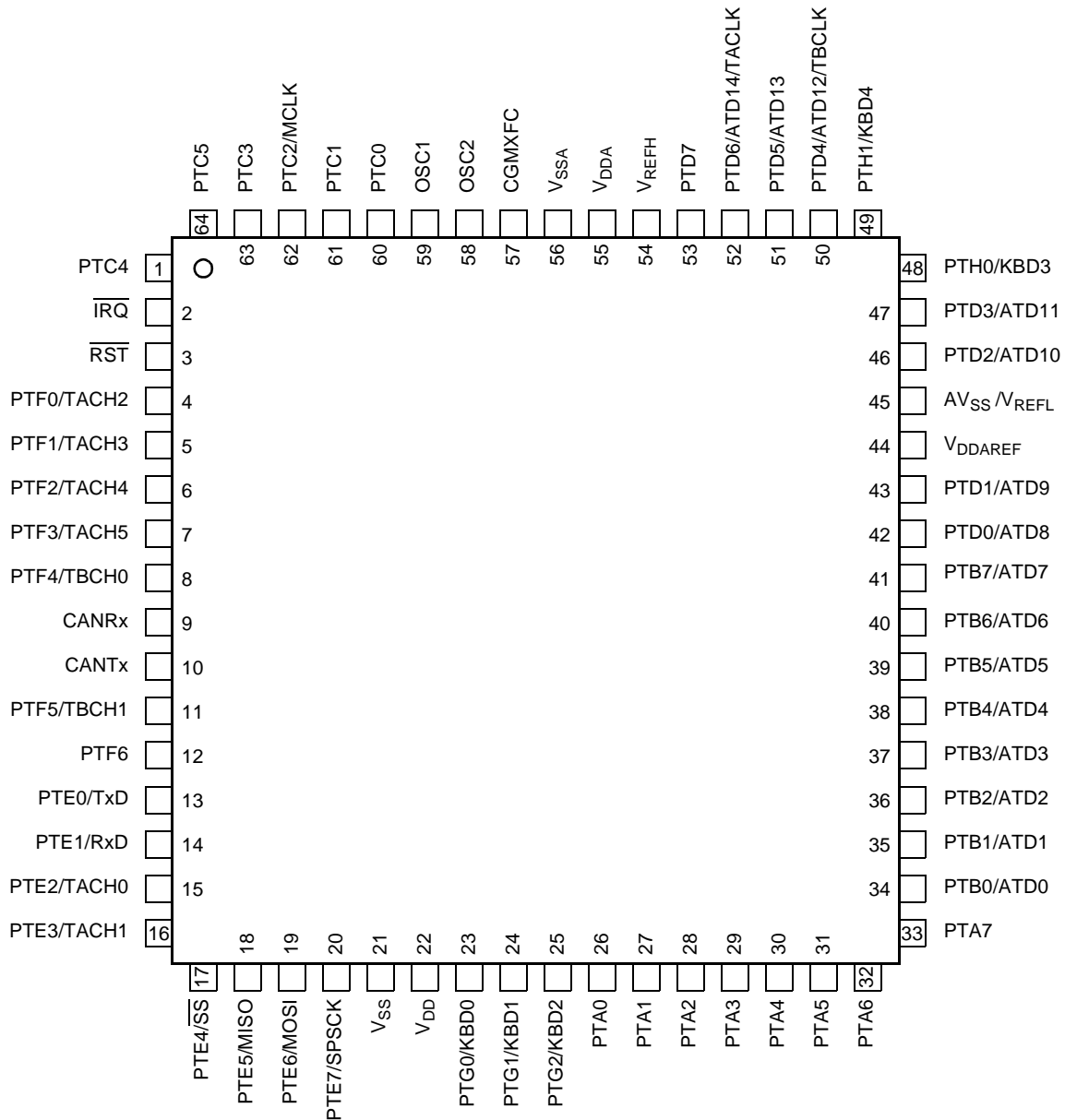
Figure 2. MC68HC08AZ60 (64-Pin QFP)
