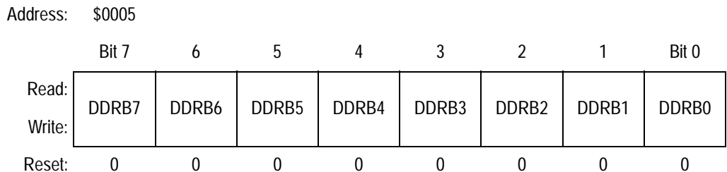
Figure 6. Data Direction Register B (DDRB)
