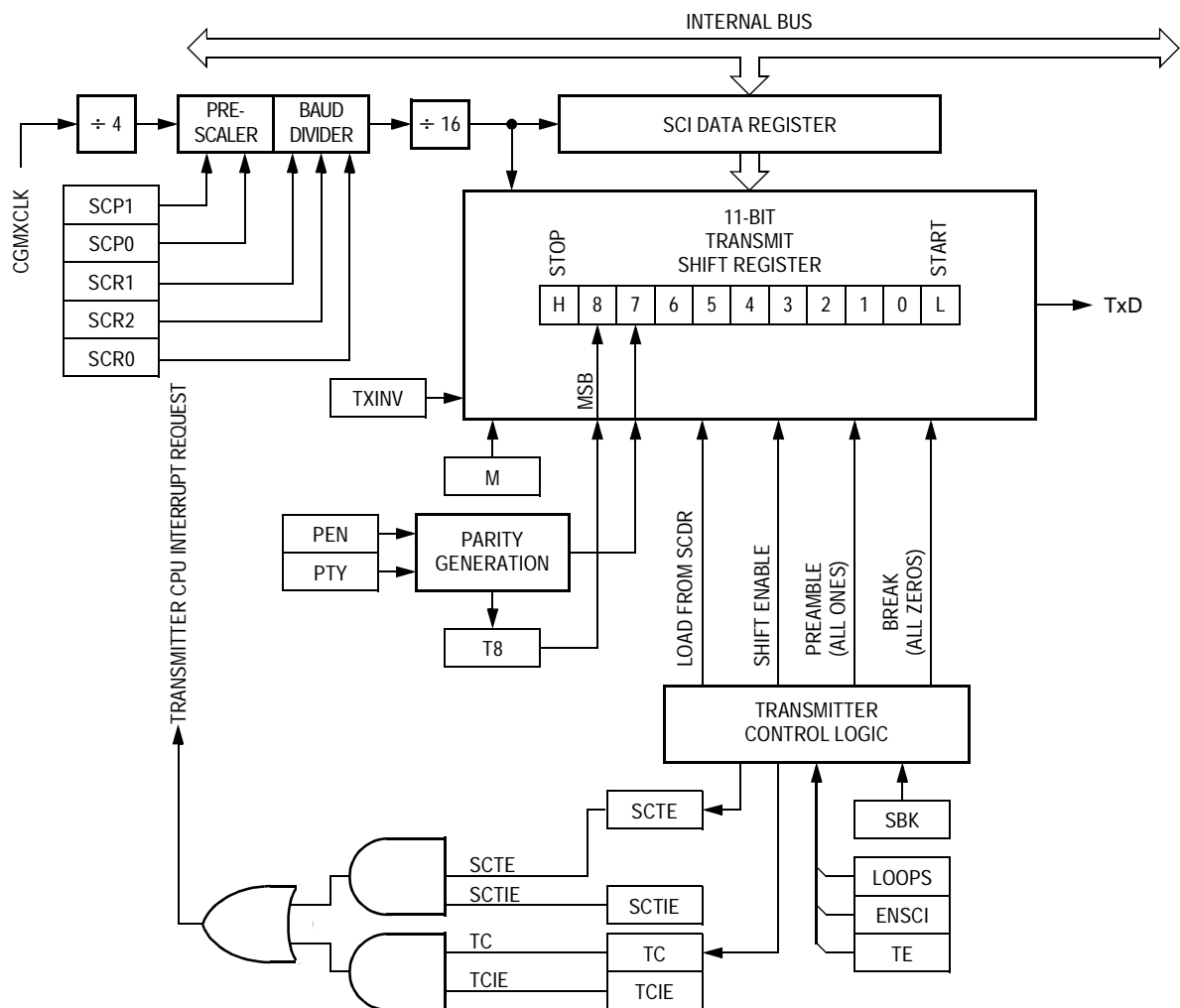
Figure 4. SCI Transmitter
