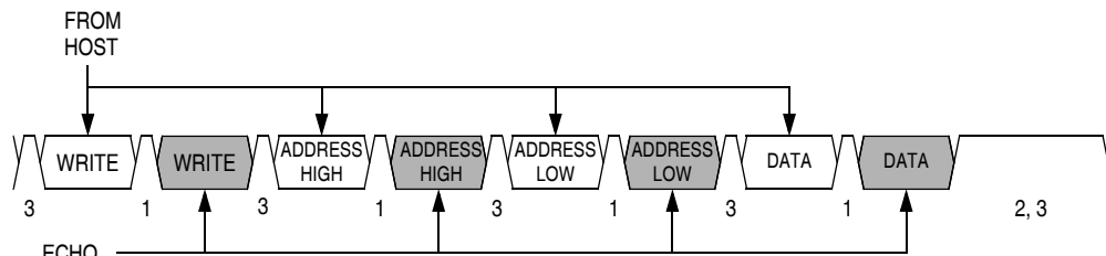
Figure 15-13. Read Transaction
