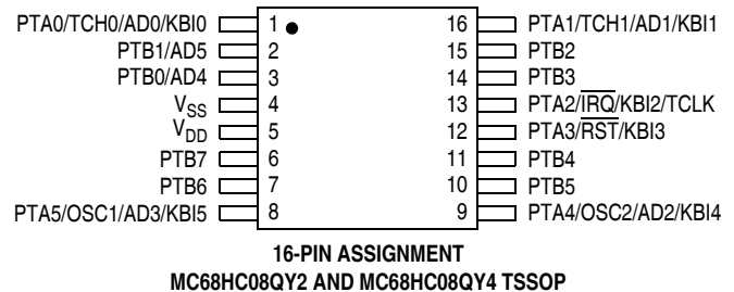
Figure 1-2. MCU Pin Assignments
