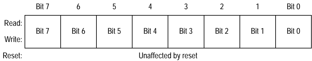
Figure 9-22. Pulse Accumulator Counter Register (PACNT)
