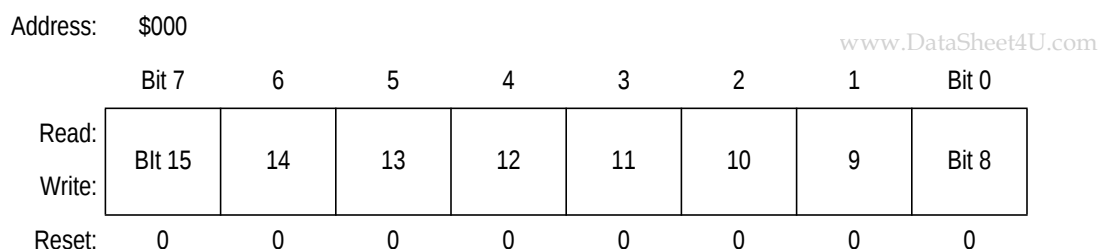
Figure 3-1. DSI Channel 0 Data Register Upper Byte (DSI0H)
