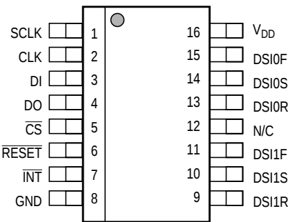
16-lead narrow body SOIC, package #751B-05 issue J
