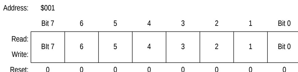
Figure 3-2. DSI Channel 0 Data Register Lower Byte (DSI0L)
