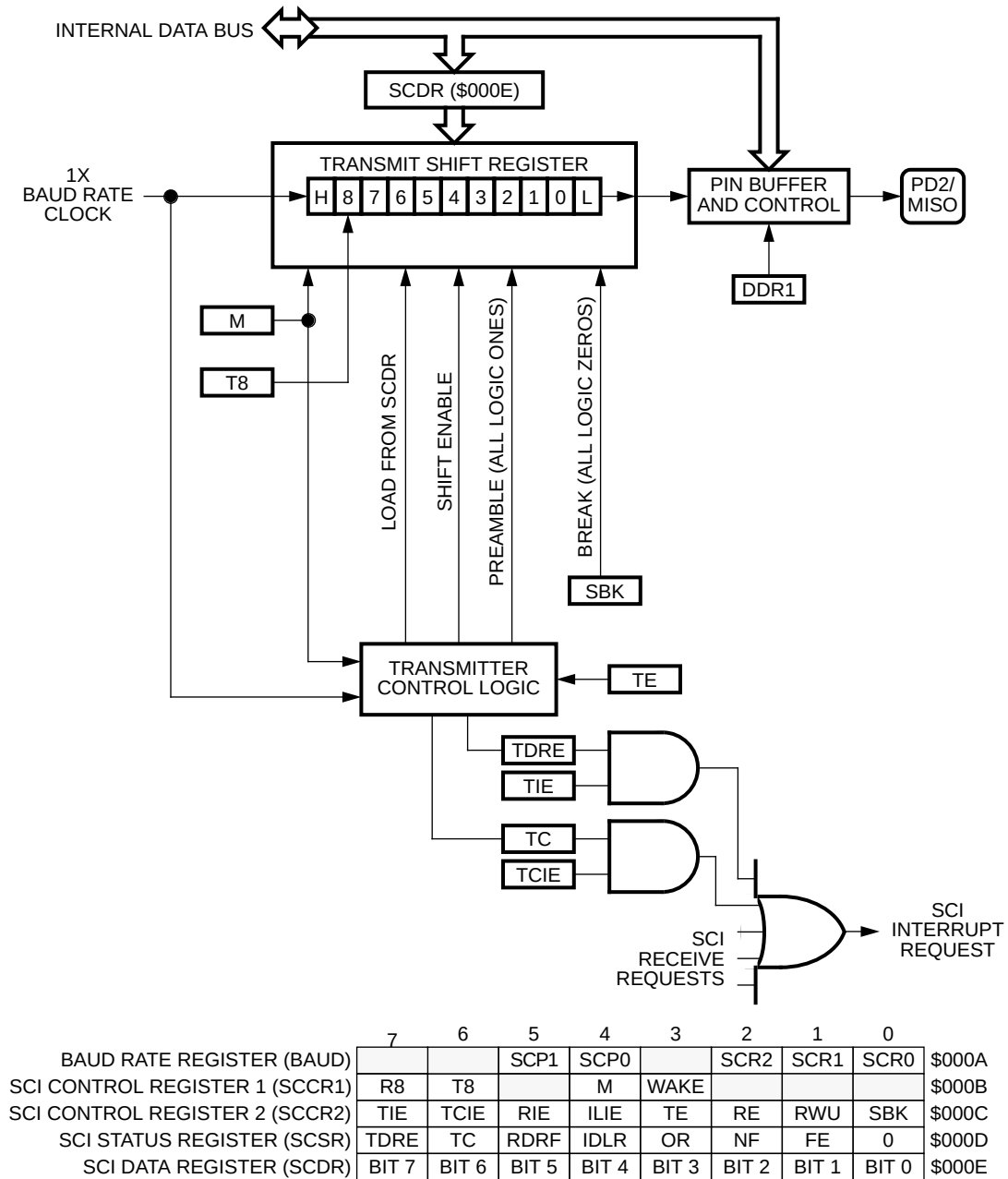
Figure 10-2: SCI Transmitter
