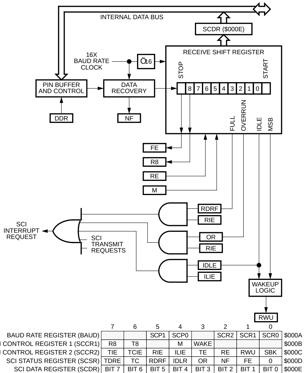
Figure 10-3: SCI Receiver
