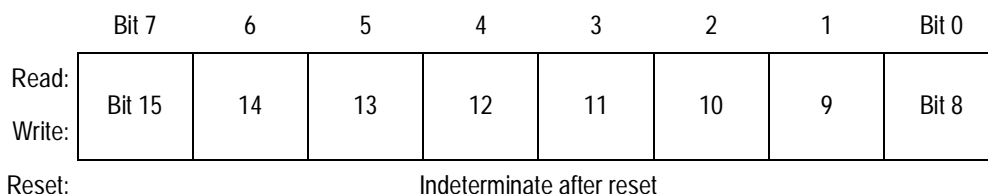
Figure 22-9. TIMA Channel Registers (TACH0H/L–TACH3H/L) (Sheet 1 of 3)
