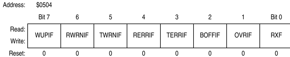
Figure 24-19. Receiver Flag Register (CRFLG)
