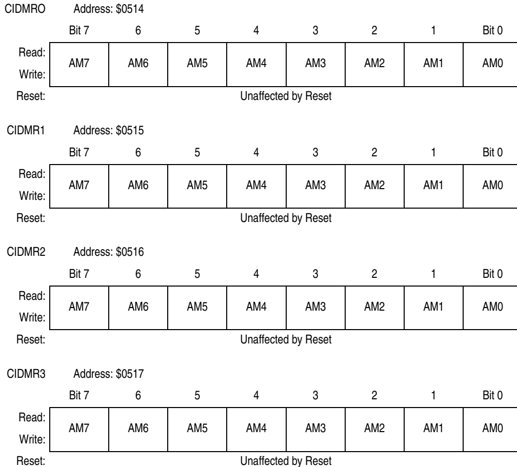
Figure 24-27. Identifier Mask Registers (CIDMR0–CIDMR3)
