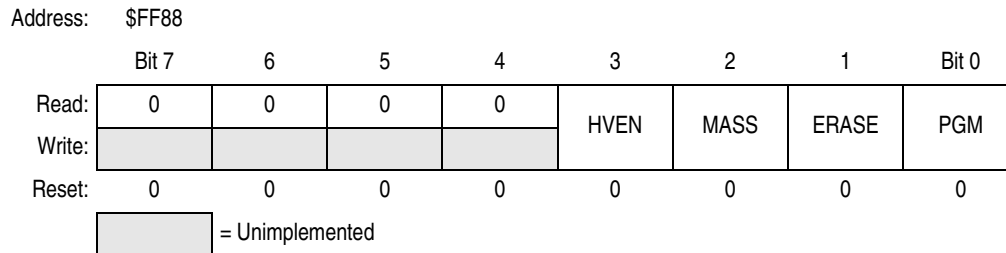
Figure 4-1. FLASH Control Register (FLCR)
