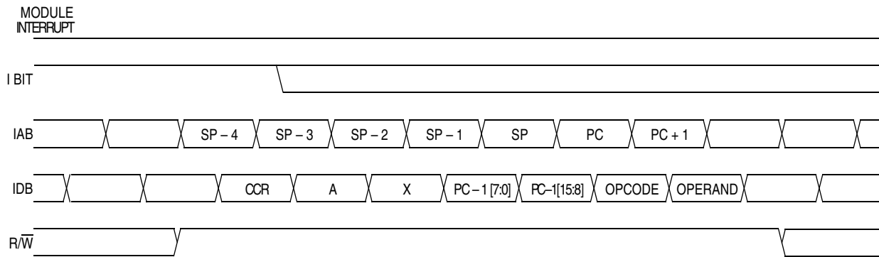
Figure 7-9. Interrupt Recovery
