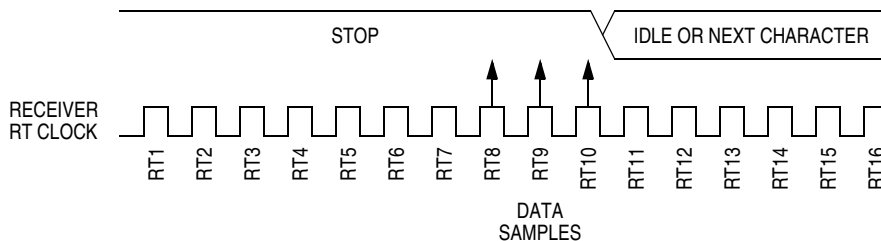
Figure 16-10. Fast Data
