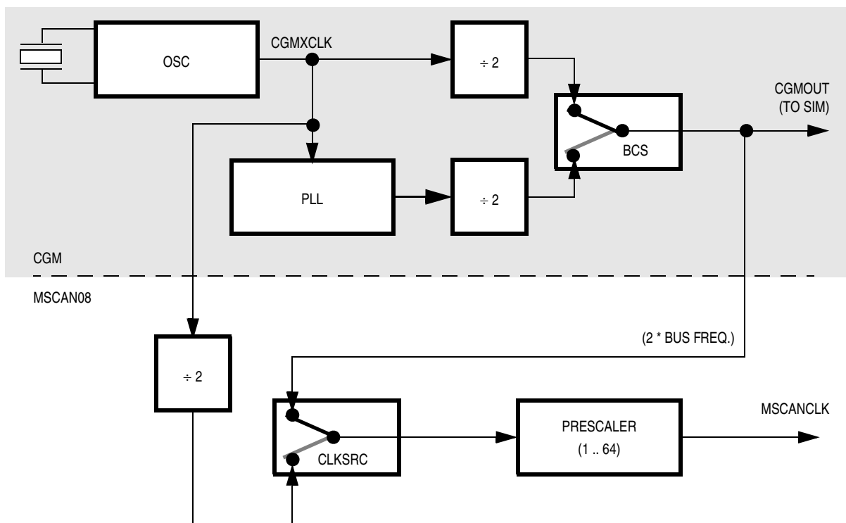
Figure 24-7. Clocking Scheme
