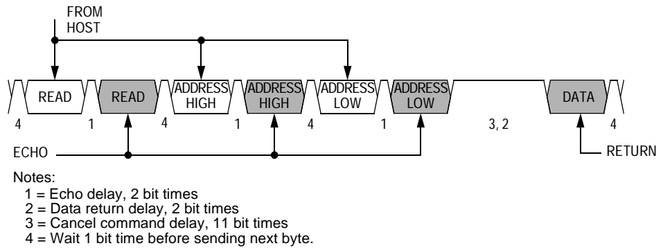
Figure 10-4. Read Transaction
