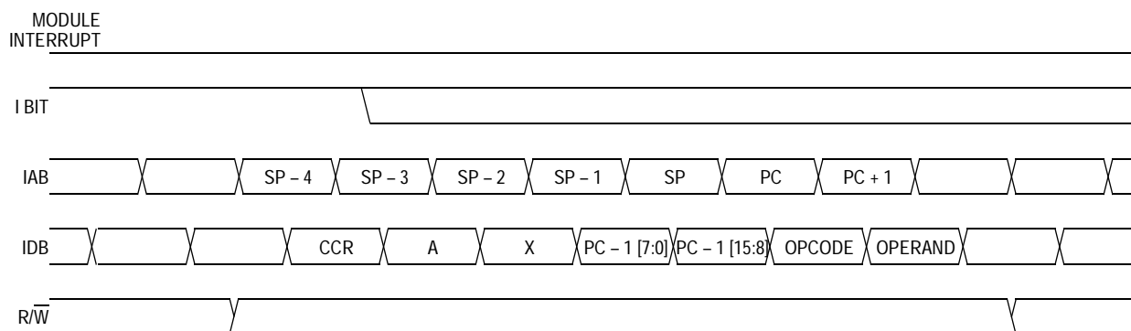
Figure 6-8. Interrupt Recovery
