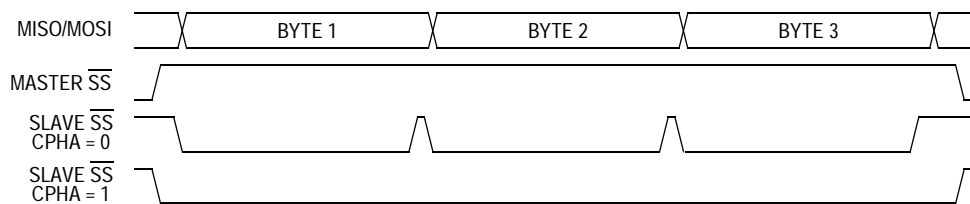
Figure 15-10. CPHA/SS Timing
