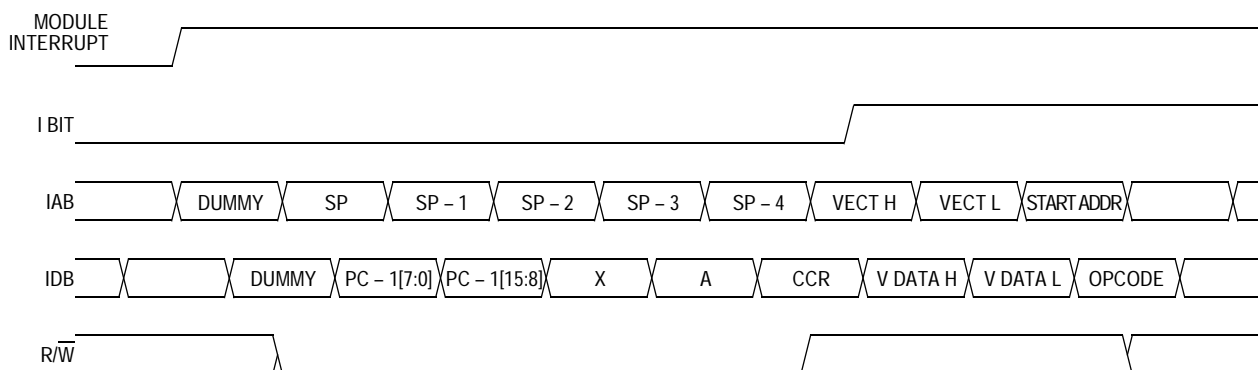
Figure 6-7. Interrupt Entry
