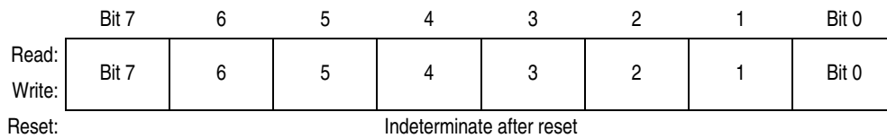
Figure 19-14. TIM Channel 0 Register Low (TCH0L)
