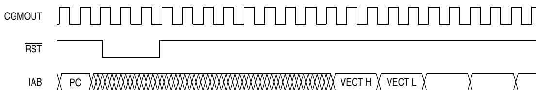
Figure 16-4. External Reset Timing
