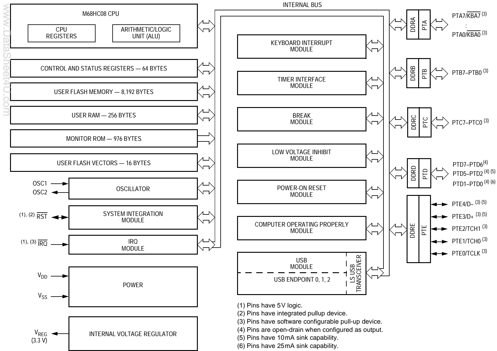
Figure 1-1. MCU Block Diagram
