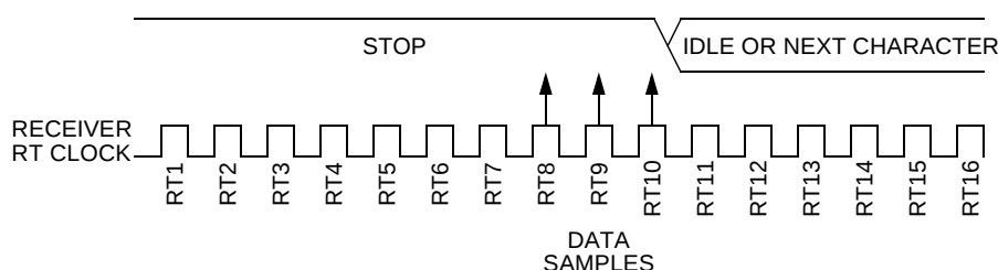
Figure 12-8. Fast Data
