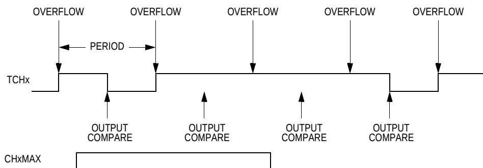
Figure 10-11. CHxMAX Latency
