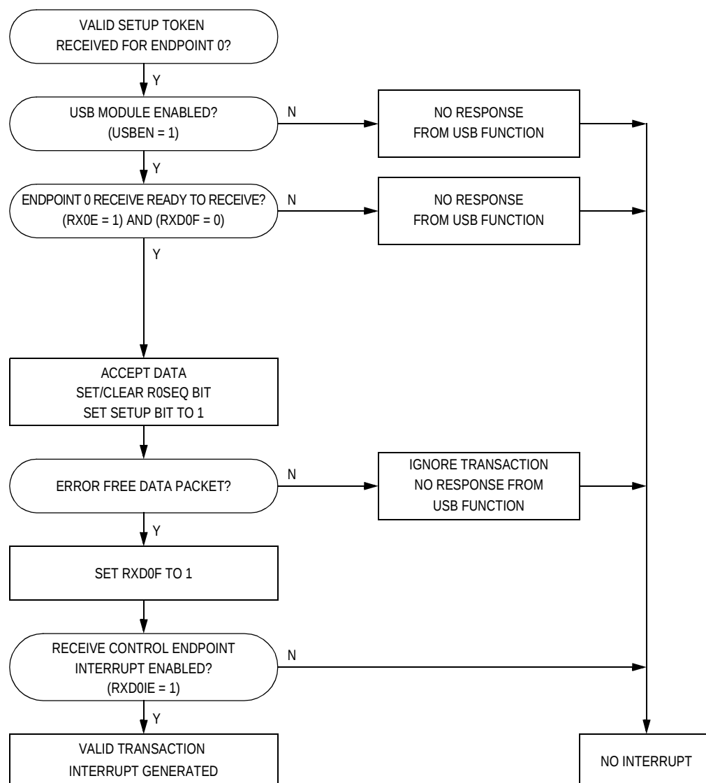
Figure 11-30. SETUP Token Data Flow for Receive Endpoint 0
