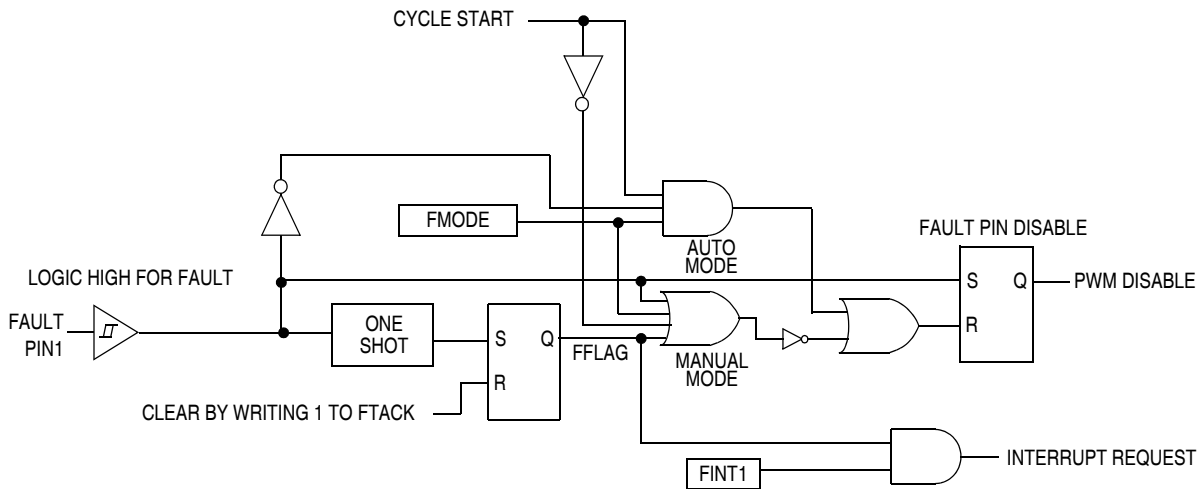
Figure 15-10. PWM Disabling Scheme
