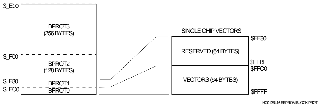
Figure 11 EEPROM Block Protect Mapping
