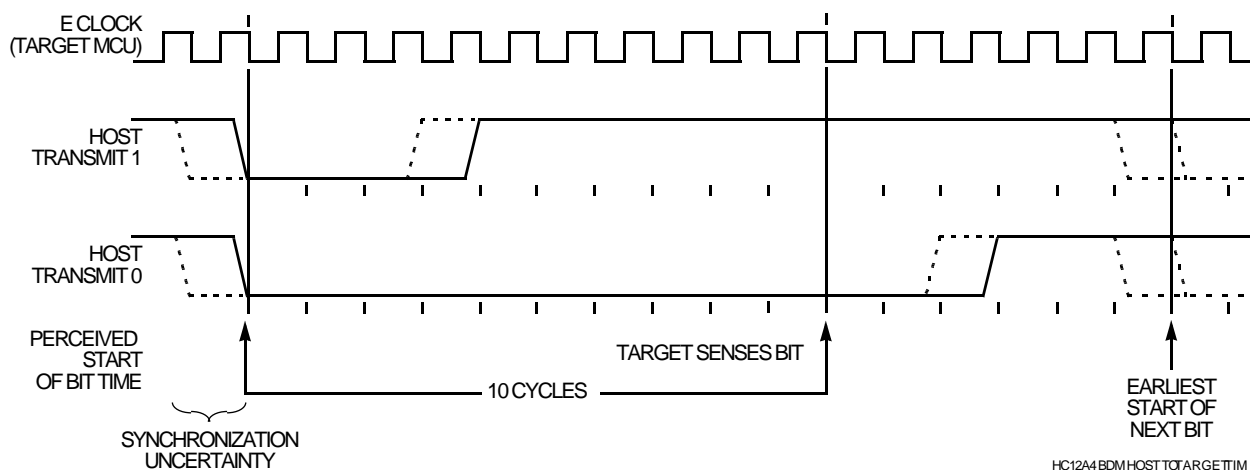
Figure 28 BDM Host to Target Serial Bit Timing
