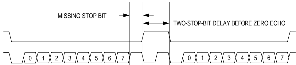
Figure 9-5. Break Transaction
