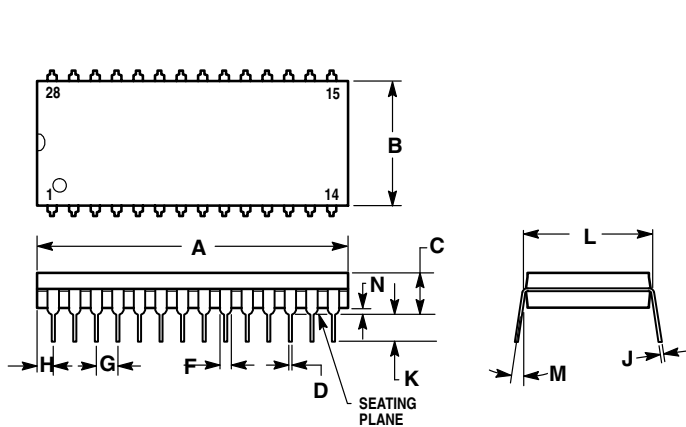
Figure 17-3. 28-Pin PDIP (Case #710)
