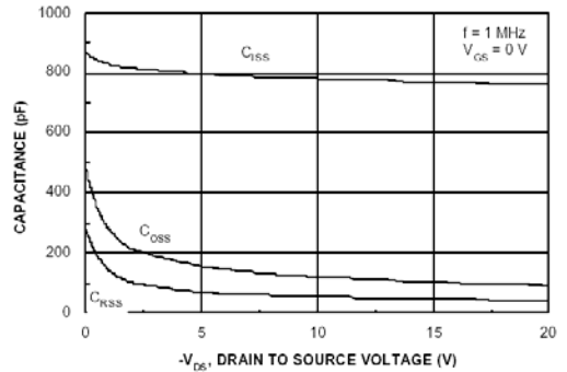
Figure 8. Capacitance Characteristic
