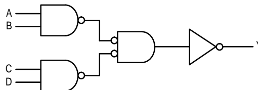
EXPANDED LOGIC DIAGRAM (1/2 OF THE DEVICE)
